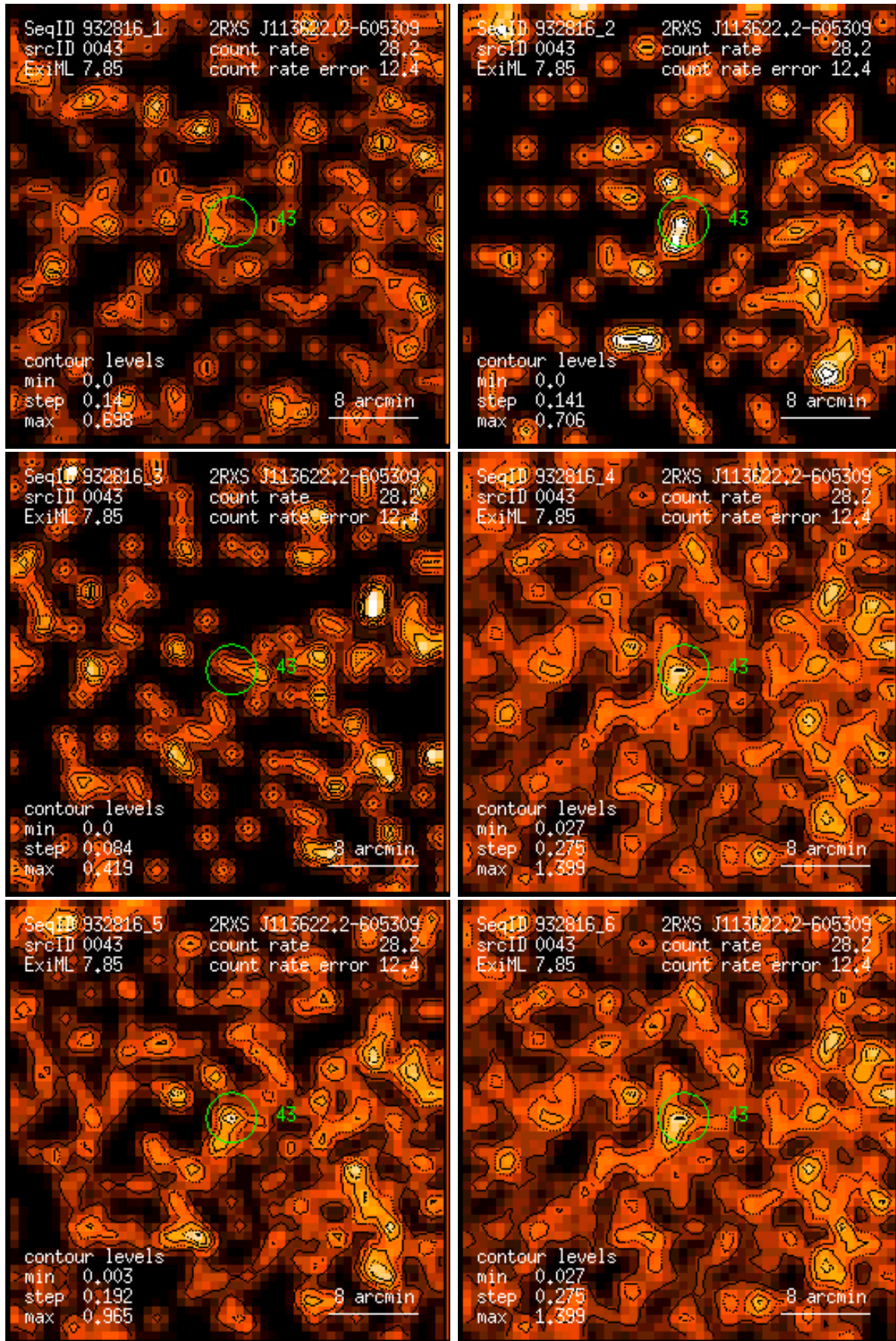
Figure 43: RASS 932816: detection 0043: band rate images, Gaussian filter: (1) PSPC channels 11 – 41, (2) 52 – 90, (3) 91 – 201, (4) 11 – 235, (5) 52 – 201, (6) 11 – 201. Broad band rates in counts/ks. Band rate contour levels in counts/ks/arcmin 2 .
