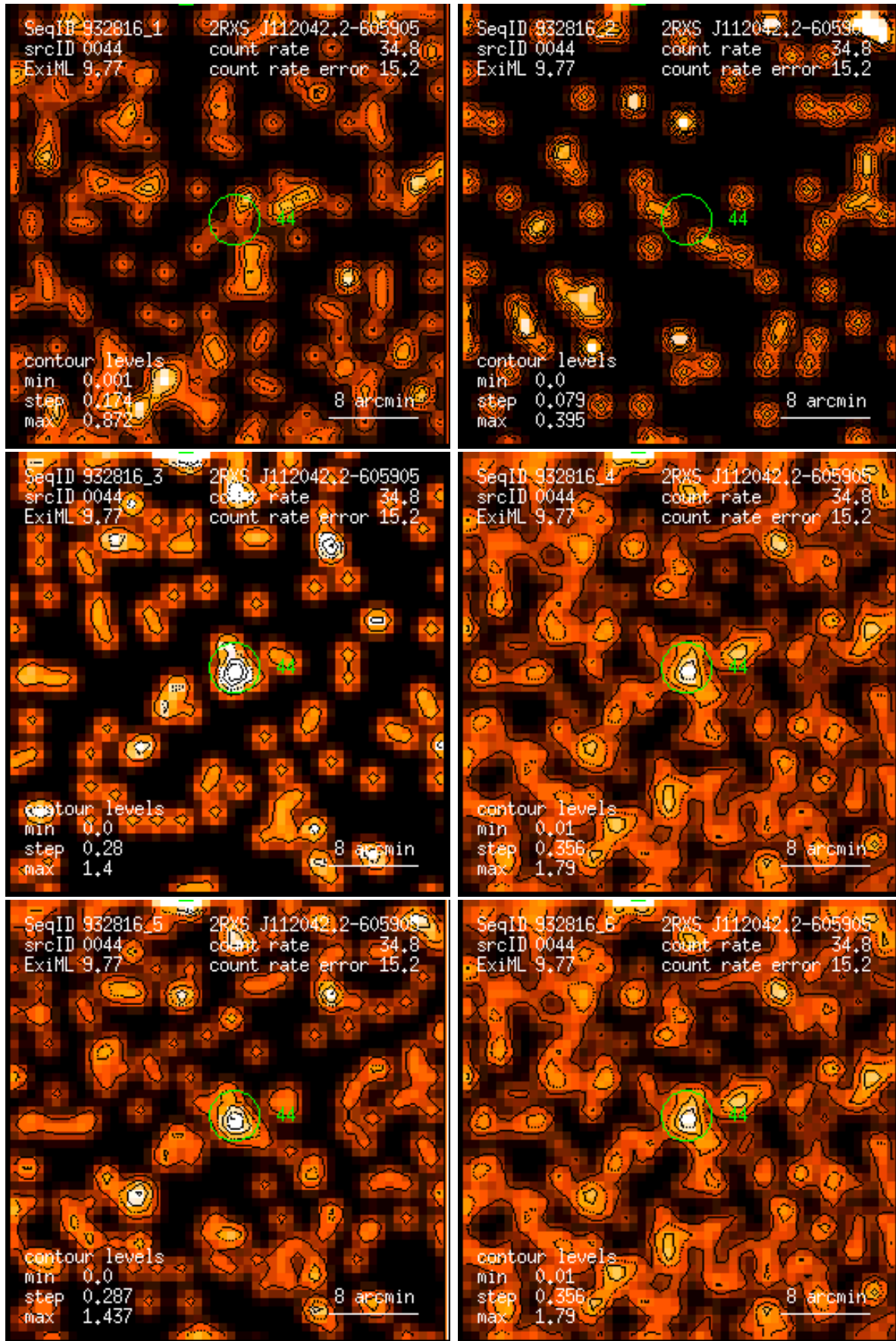
Figure 44: RASS 932816: detection 0044: band rate images, Gaussian filter: (1) PSPC channels 11 – 41, (2) 52 – 90, (3) 91 – 201, (4) 11 – 235, (5) 52 – 201, (6) 11 – 201. Broad band rates in counts/ks. Band rate contour levels in counts/ks/arcmin 2 .
