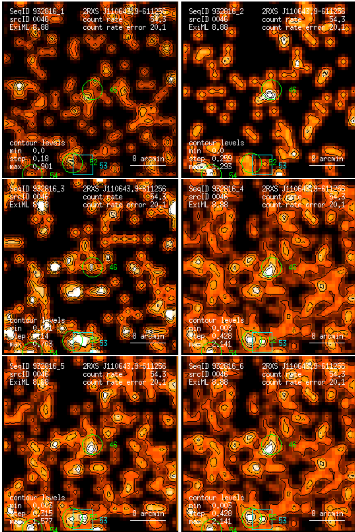
Figure 46: RASS 932816: detection 0046: band rate images, Gaussian filter: (1) PSPC channels 11 – 41, (2) 52 – 90, (3) 91 – 201, (4) 11 – 235, (5) 52 – 201, (6) 11 – 201. Broad band rates in counts/ks. Band rate contour levels in counts/ks/arcmin 2 .
