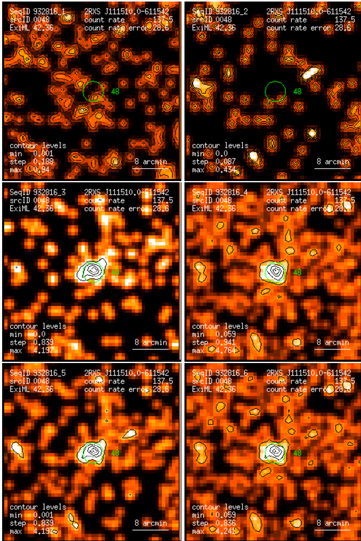
Figure 48: RASS 932816: detection 0048: band rate images, Gaussian filter: (1) PSPC channels 11 – 41, (2) 52 – 90, (3) 91 – 201, (4) 11 – 235, (5) 52 – 201, (6) 11 – 201. Broad band rates in counts/ks. Band rate contour levels in counts/ks/arcmin 2 .
