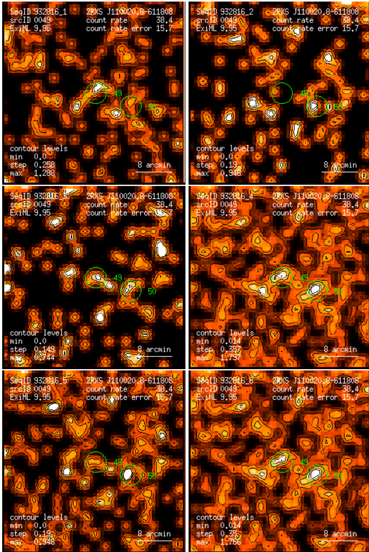
Figure 49: RASS 932816: detection 0049: band rate images, Gaussian filter: (1) PSPC channels 11 – 41, (2) 52 – 90, (3) 91 – 201, (4) 11 – 235, (5) 52 – 201, (6) 11 – 201. Broad band rates in counts/ks. Band rate contour levels in counts/ks/arcmin 2 .
