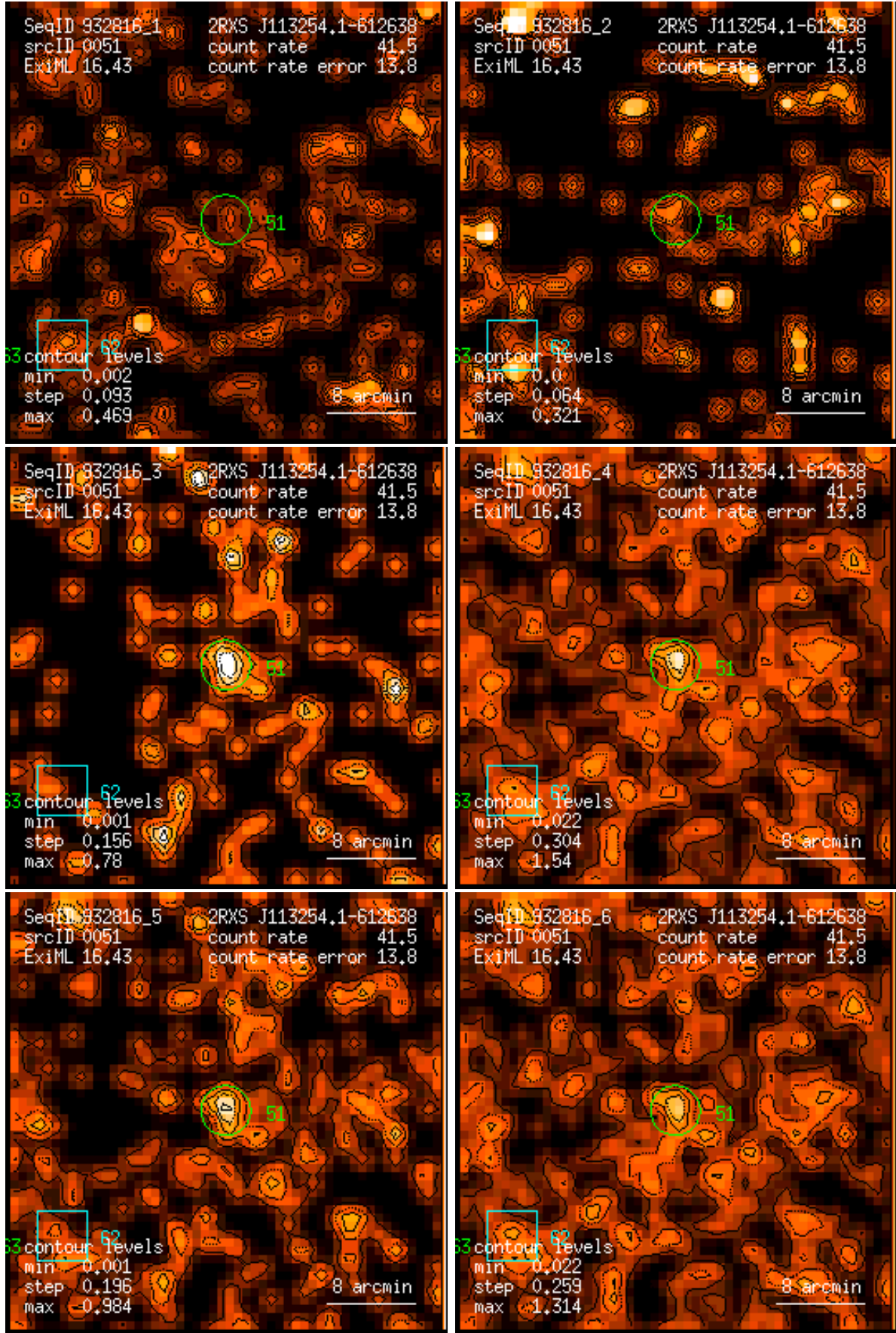
Figure 51: RASS 932816: detection 0051: band rate images, Gaussian filter: (1) PSPC channels 11 – 41, (2) 52 – 90, (3) 91 – 201, (4) 11 – 235, (5) 52 – 201, (6) 11 – 201. Broad band rates in counts/ks. Band rate contour levels in counts/ks/arcmin 2 .
