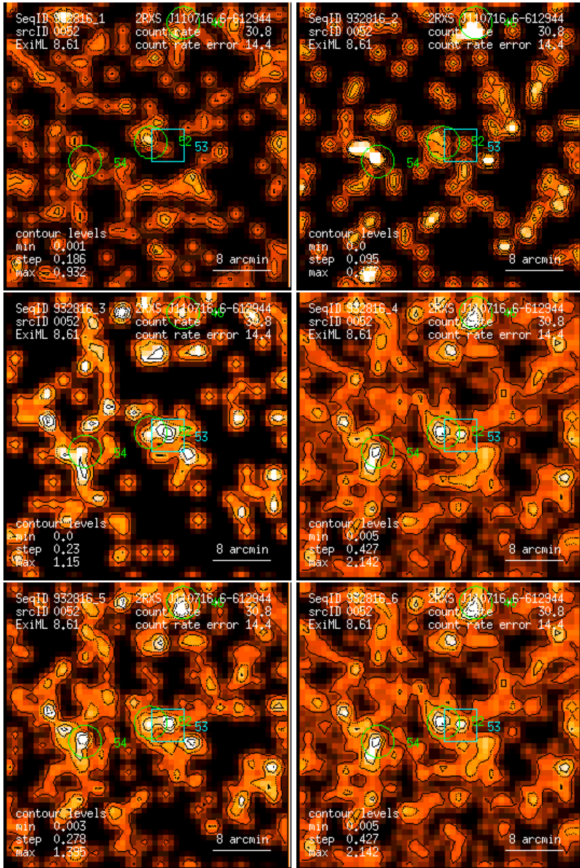
Figure 52: RASS 932816: detection 0052: band rate images, Gaussian filter: (1) PSPC channels 11 – 41, (2) 52 – 90, (3) 91 – 201, (4) 11 – 235, (5) 52 – 201, (6) 11 – 201. Broad band rates in counts/ks. Band rate contour levels in counts/ks/arcmin 2 .
