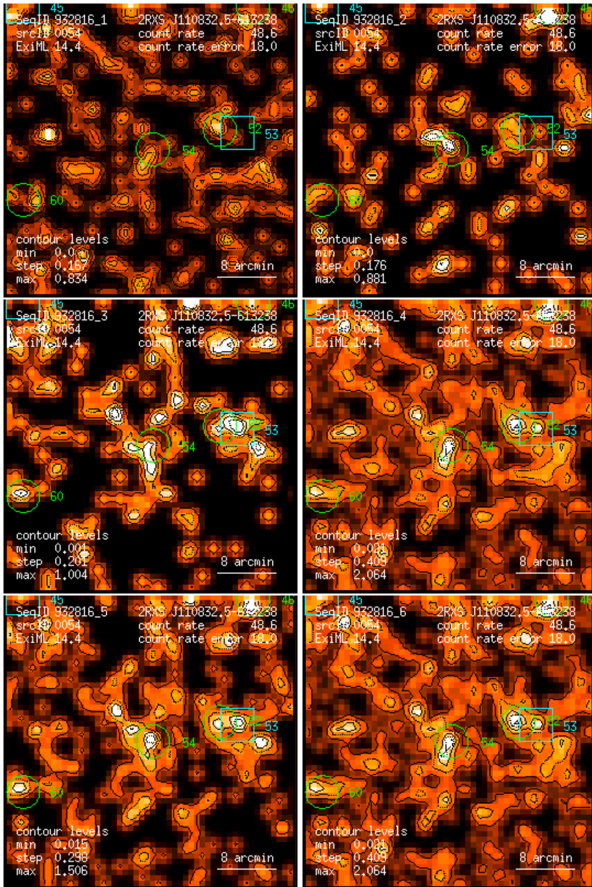
Figure 54: RASS 932816: detection 0054: band rate images, Gaussian filter: (1) PSPC channels 11 – 41, (2) 52 – 90, (3) 91 – 201, (4) 11 – 235, (5) 52 – 201, (6) 11 – 201. Broad band rates in counts/ks. Band rate contour levels in counts/ks/arcmin 2 .
