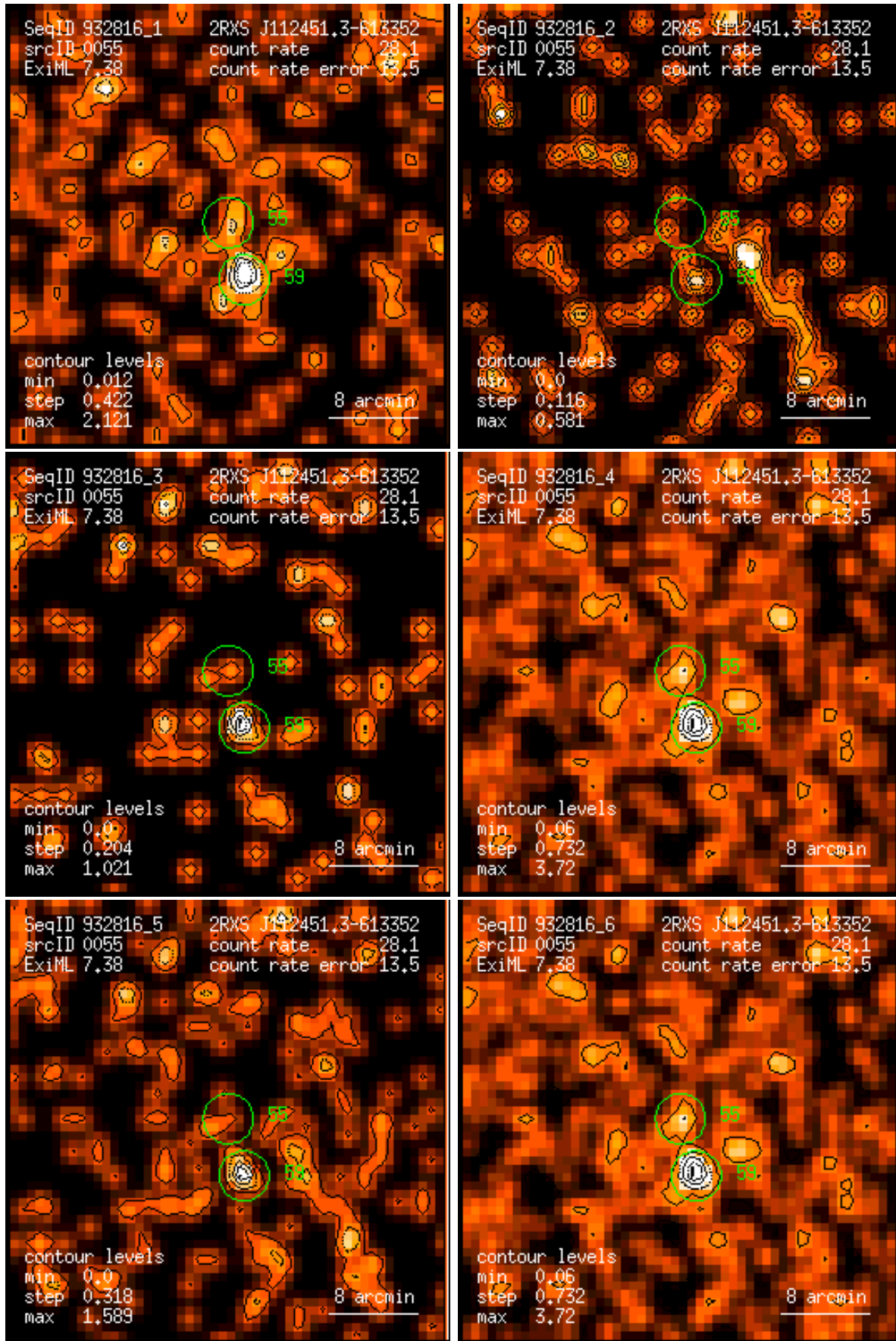
Figure 55: RASS 932816: detection 0055: band rate images, Gaussian filter: (1) PSPC channels 11 – 41, (2) 52 – 90, (3) 91 – 201, (4) 11 – 235, (5) 52 – 201, (6) 11 – 201. Broad band rates in counts/ks. Band rate contour levels in counts/ks/arcmin 2 .
