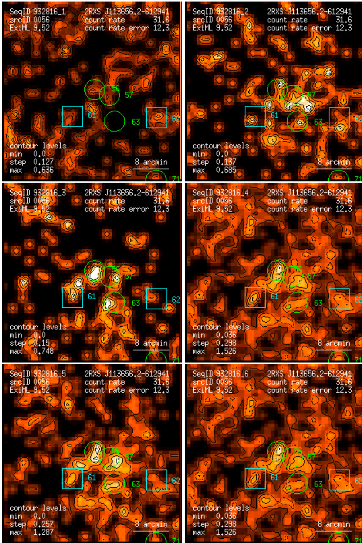
Figure 56: RASS 932816: detection 0056: band rate images, Gaussian filter: (1) PSPC channels 11 – 41, (2) 52 – 90, (3) 91 – 201, (4) 11 – 235, (5) 52 – 201, (6) 11 – 201. Broad band rates in counts/ks. Band rate contour levels in counts/ks/arcmin 2 .
