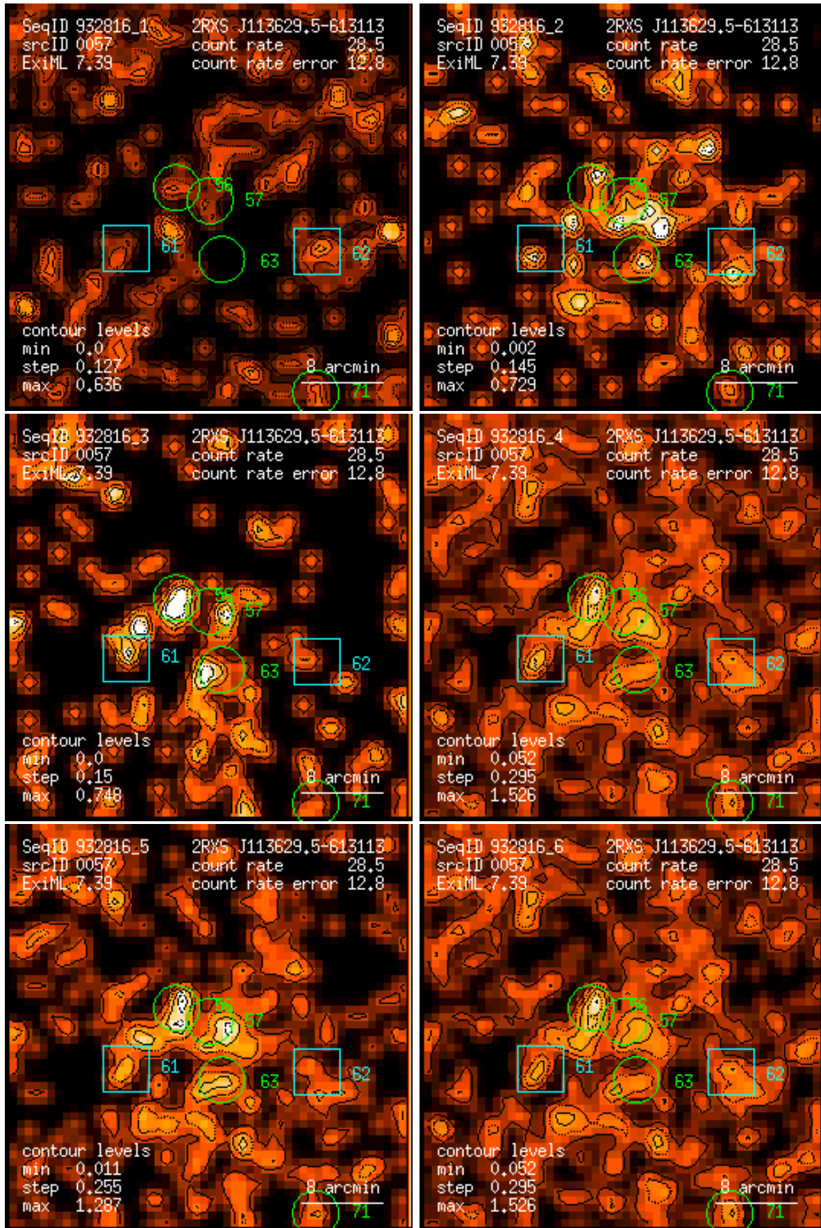
Figure 57: RASS 932816: detection 0057: band rate images, Gaussian filter: (1) PSPC channels 11 – 41, (2) 52 – 90, (3) 91 – 201, (4) 11 – 235, (5) 52 – 201, (6) 11 – 201. Broad band rates in counts/ks. Band rate contour levels in counts/ks/arcmin 2 .
