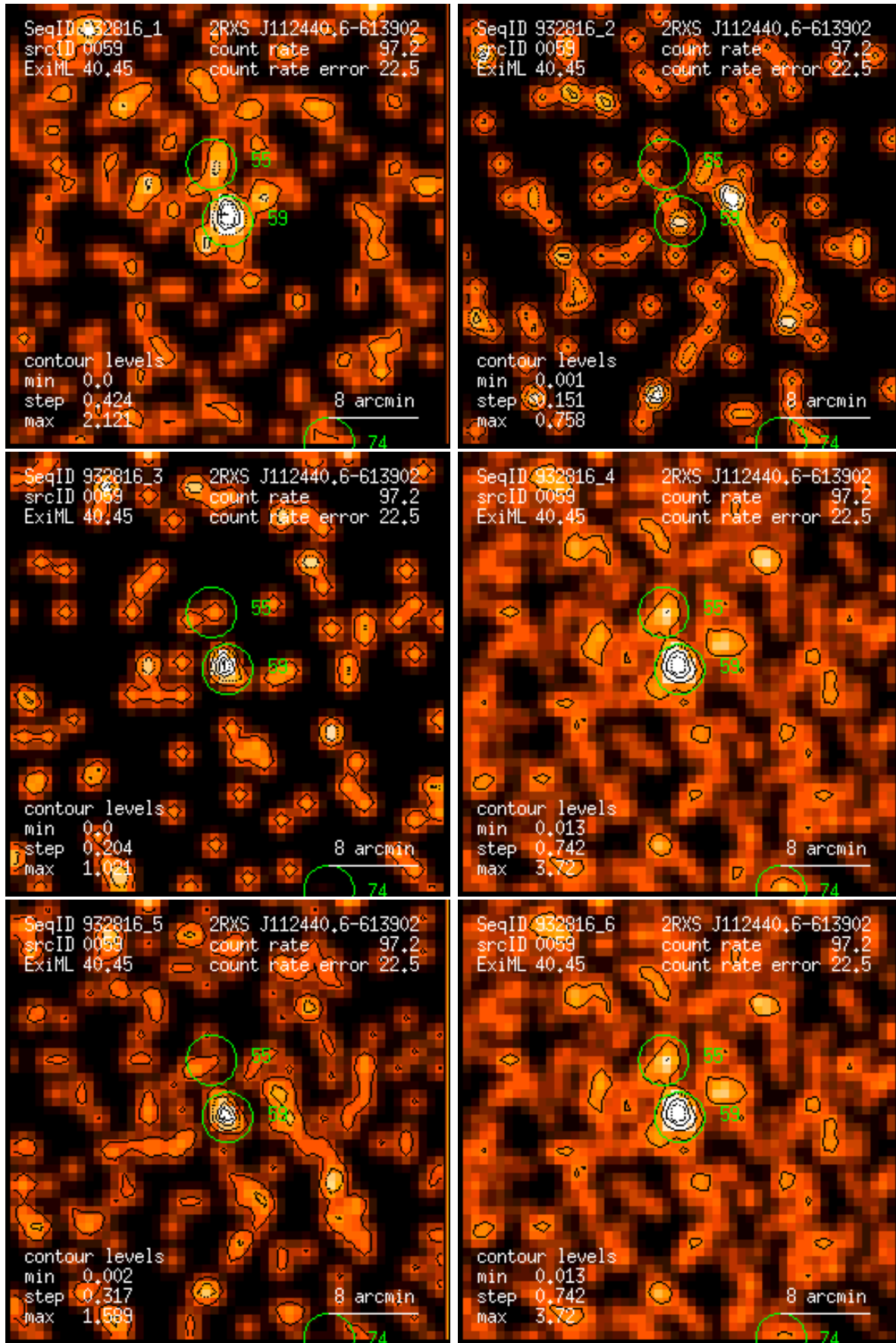
Figure 59: RASS 932816: detection 0059: band rate images, Gaussian filter: (1) PSPC channels 11 – 41, (2) 52 – 90, (3) 91 – 201, (4) 11 – 235, (5) 52 – 201, (6) 11 – 201. Broad band rates in counts/ks. Band rate contour levels in counts/ks/arcmin 2 .
