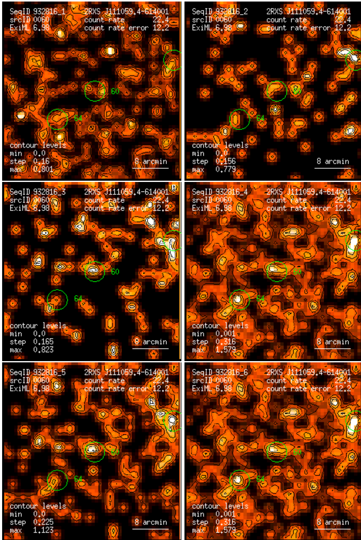
Figure 60: RASS 932816: detection 0060: band rate images, Gaussian filter: (1) PSPC channels 11 – 41, (2) 52 – 90, (3) 91 – 201, (4) 11 – 235, (5) 52 – 201, (6) 11 – 201. Broad band rates in counts/ks. Band rate contour levels in counts/ks/arcmin 2 .
