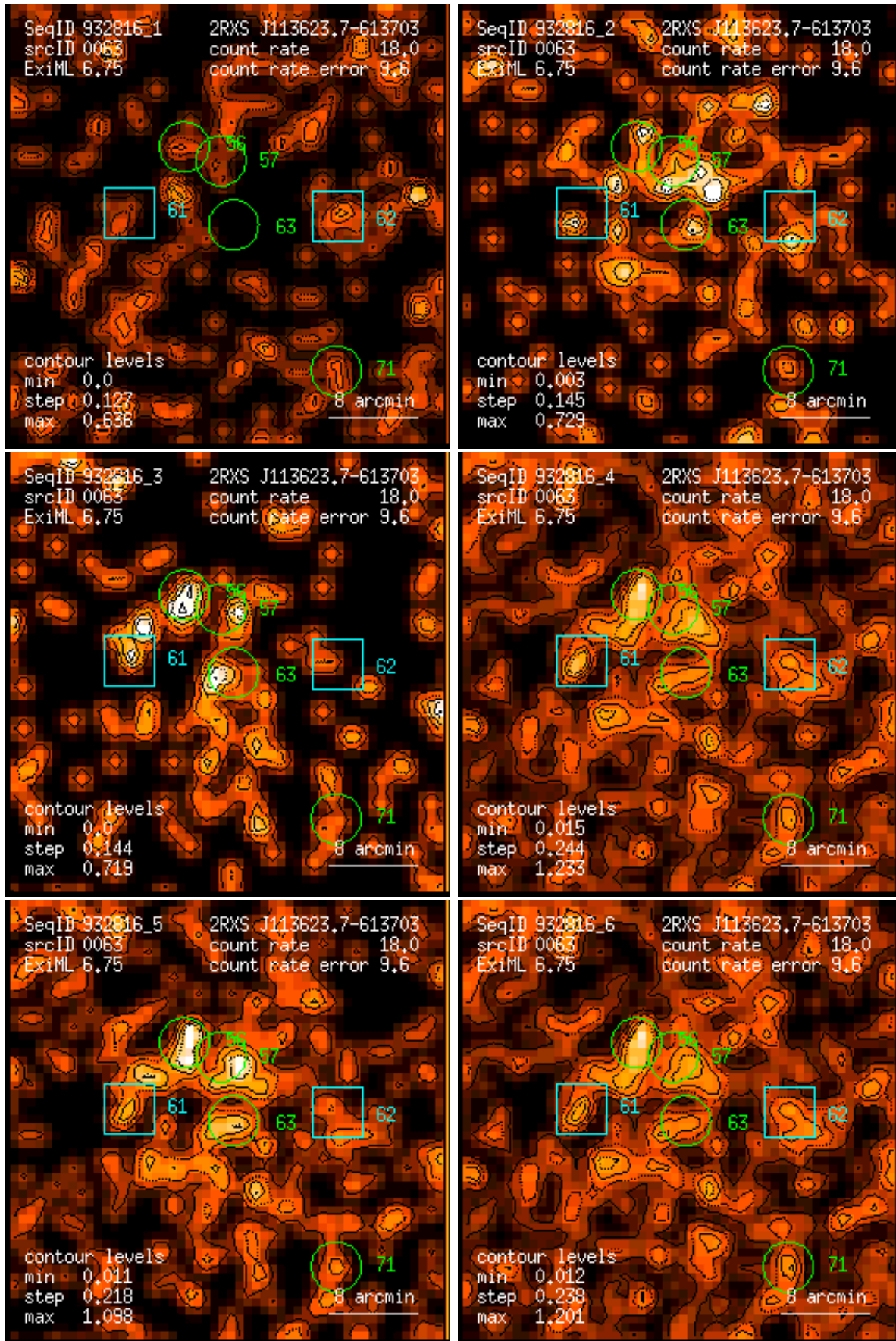
Figure 63: RASS 932816: detection 0063: band rate images, Gaussian filter: (1) PSPC channels 11 – 41, (2) 52 – 90, (3) 91 – 201, (4) 11 – 235, (5) 52 – 201, (6) 11 – 201. Broad band rates in counts/ks. Band rate contour levels in counts/ks/arcmin 2 .
