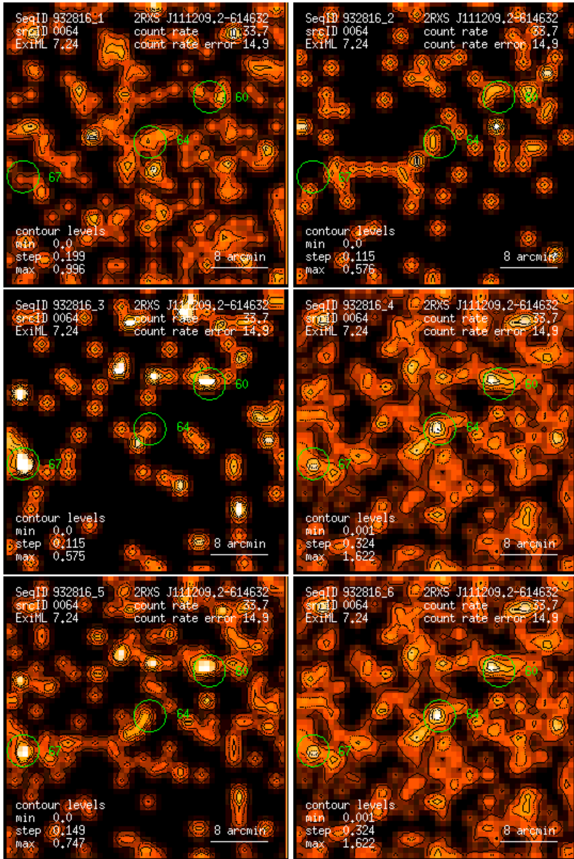
Figure 64: RASS 932816: detection 0064: band rate images, Gaussian filter: (1) PSPC channels 11 – 41, (2) 52 – 90, (3) 91 – 201, (4) 11 – 235, (5) 52 – 201, (6) 11 – 201. Broad band rates in counts/ks. Band rate contour levels in counts/ks/arcmin 2 .
