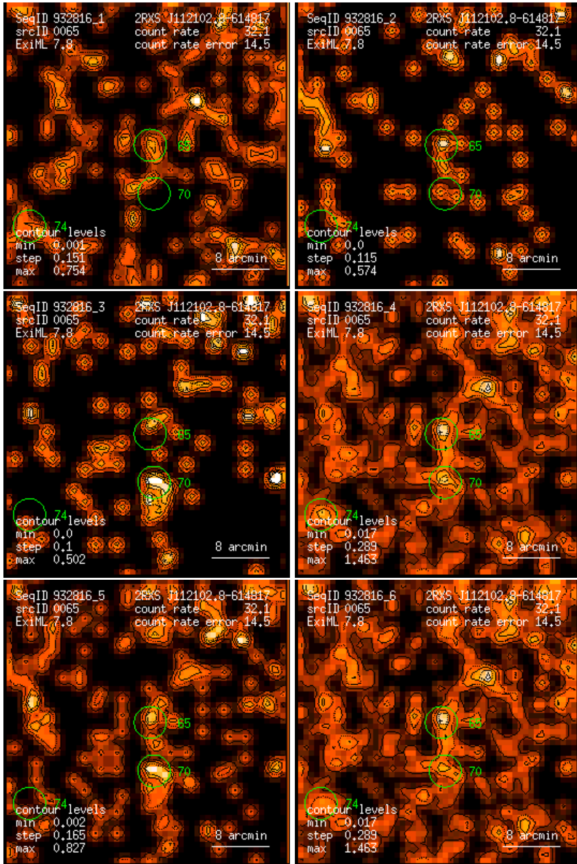
Figure 65: RASS 932816: detection 0065: band rate images, Gaussian filter: (1) PSPC channels 11 – 41, (2) 52 – 90, (3) 91 – 201, (4) 11 – 235, (5) 52 – 201, (6) 11 – 201. Broad band rates in counts/ks. Band rate contour levels in counts/ks/arcmin 2 .
