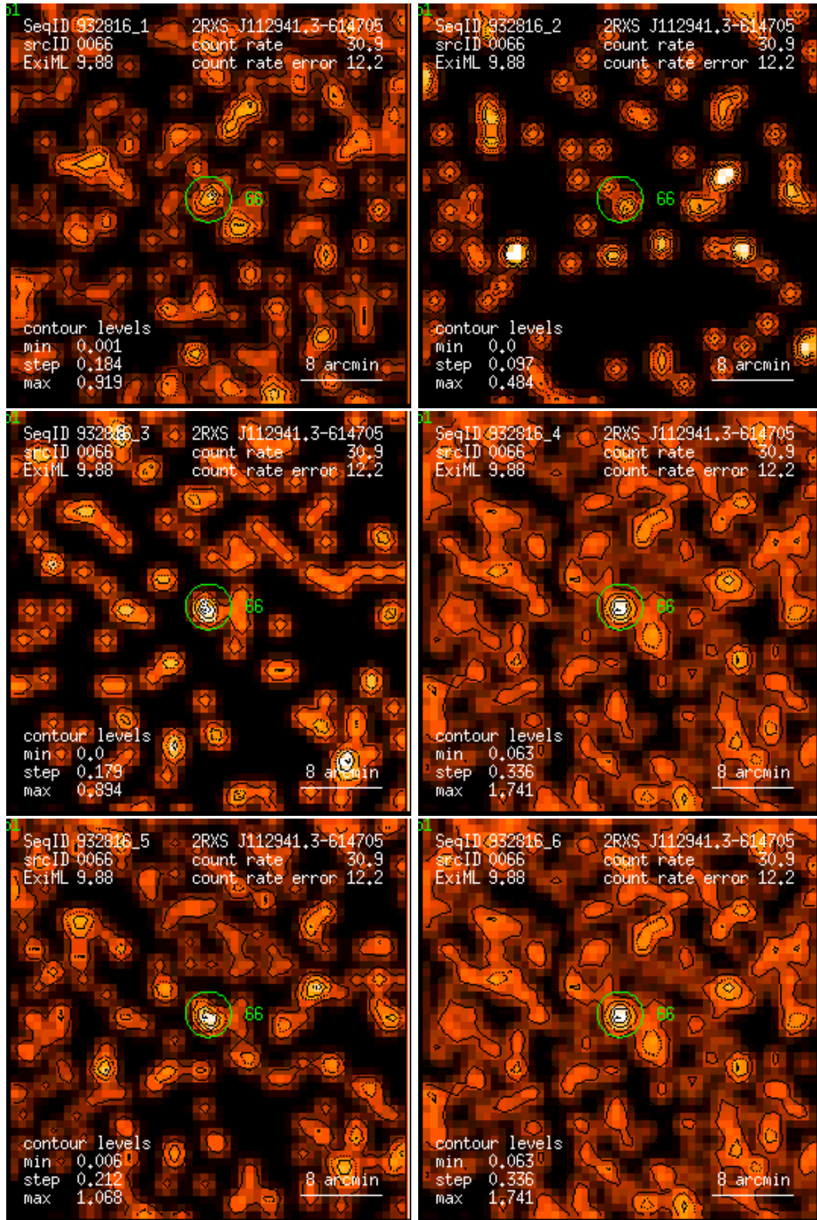
Figure 66: RASS 932816: detection 0066: band rate images, Gaussian filter: (1) PSPC channels 11 – 41, (2) 52 – 90, (3) 91 – 201, (4) 11 – 235, (5) 52 – 201, (6) 11 – 201. Broad band rates in counts/ks. Band rate contour levels in counts/ks/arcmin 2 .
