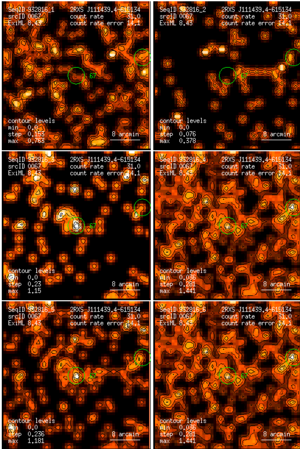
Figure 67: RASS 932816: detection 0067: band rate images, Gaussian filter: (1) PSPC channels 11 – 41, (2) 52 – 90, (3) 91 – 201, (4) 11 – 235, (5) 52 – 201, (6) 11 – 201. Broad band rates in counts/ks. Band rate contour levels in counts/ks/arcmin 2 .
