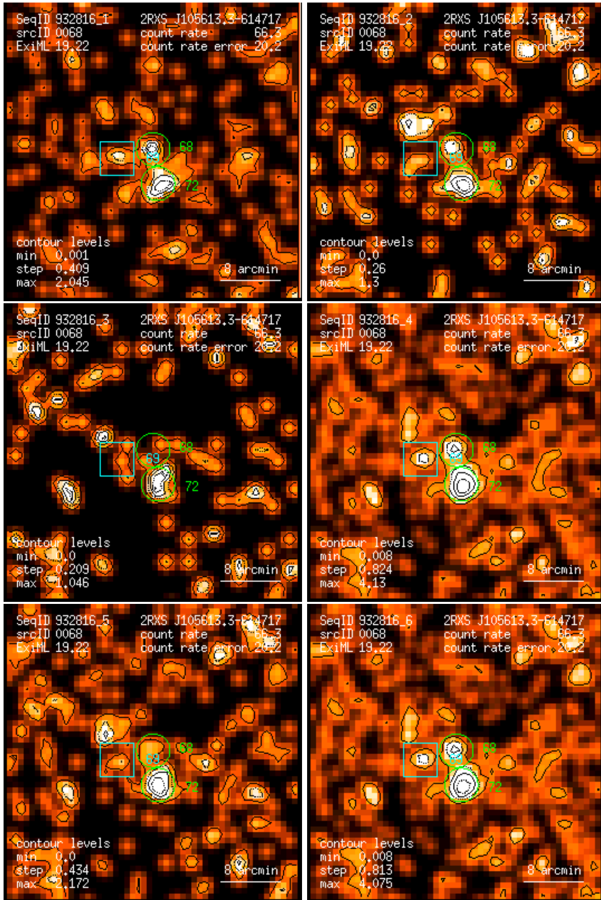
Figure 68: RASS 932816: detection 0068: band rate images, Gaussian filter: (1) PSPC channels 11 – 41, (2) 52 – 90, (3) 91 – 201, (4) 11 – 235, (5) 52 – 201, (6) 11 – 201. Broad band rates in counts/ks. Band rate contour levels in counts/ks/arcmin 2 .
