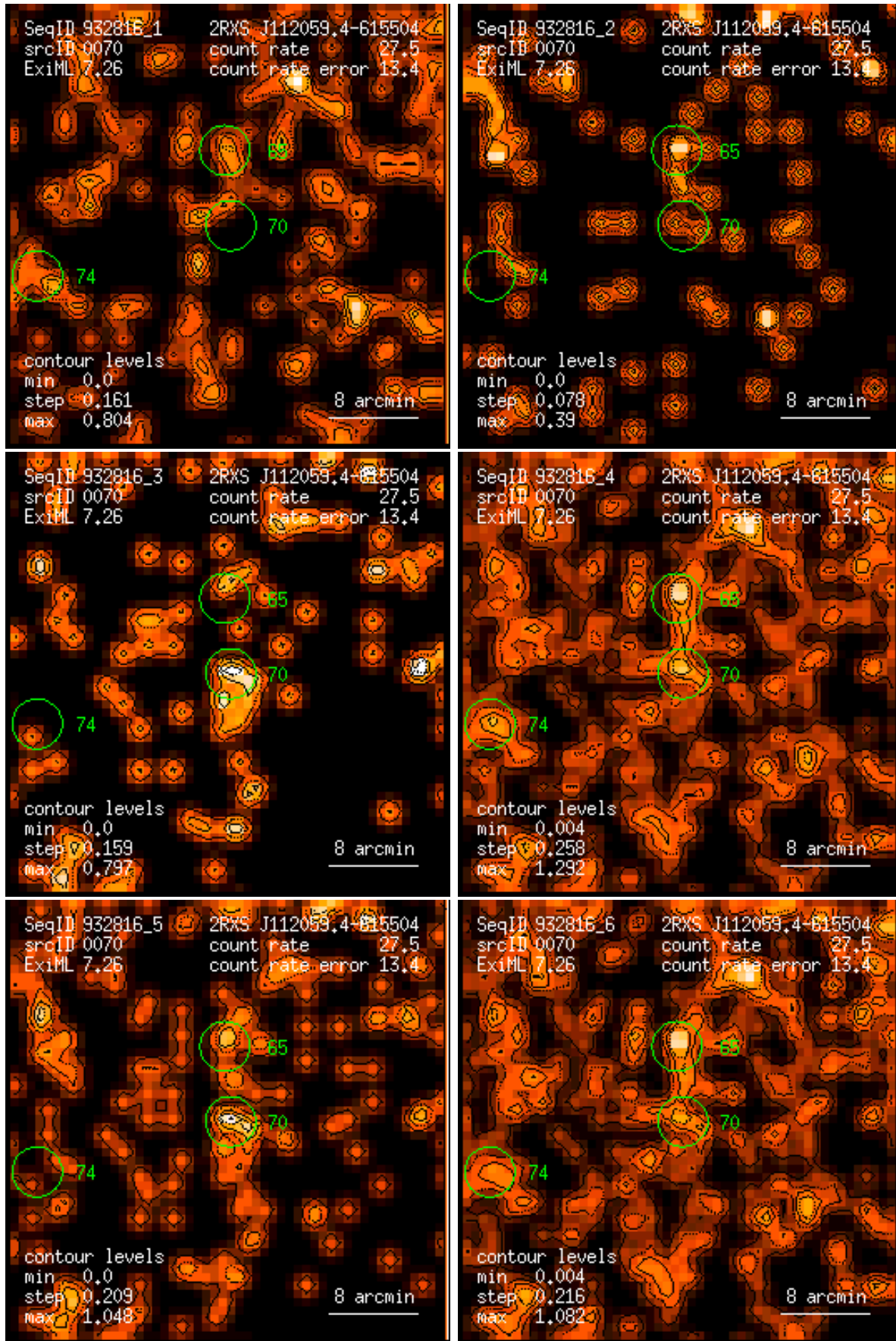
Figure 70: RASS 932816: detection 0070: band rate images, Gaussian filter: (1) PSPC channels 11 – 41, (2) 52 – 90, (3) 91 – 201, (4) 11 – 235, (5) 52 – 201, (6) 11 – 201. Broad band rates in counts/ks. Band rate contour levels in counts/ks/arcmin 2 .
