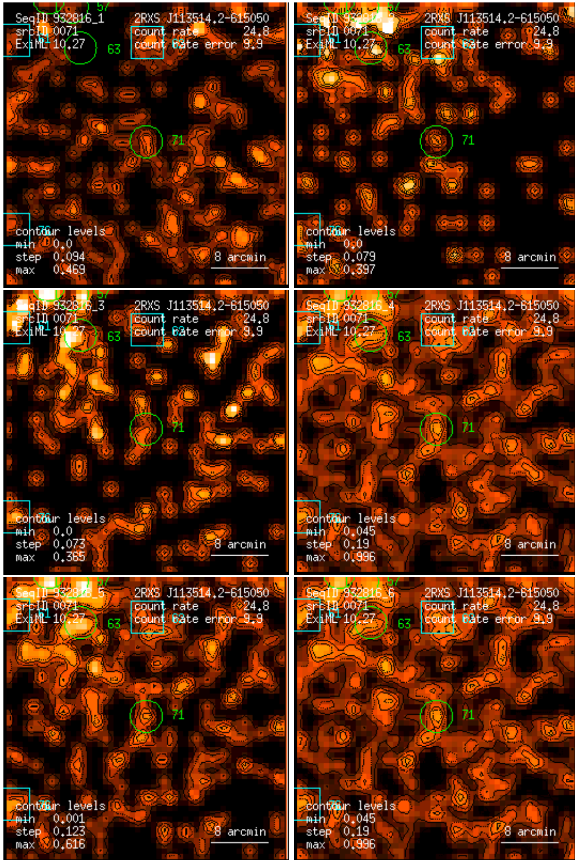
Figure 71: RASS 932816: detection 0071: band rate images, Gaussian filter: (1) PSPC channels 11 – 41, (2) 52 – 90, (3) 91 – 201, (4) 11 – 235, (5) 52 – 201, (6) 11 – 201. Broad band rates in counts/ks. Band rate contour levels in counts/ks/arcmin 2 .
