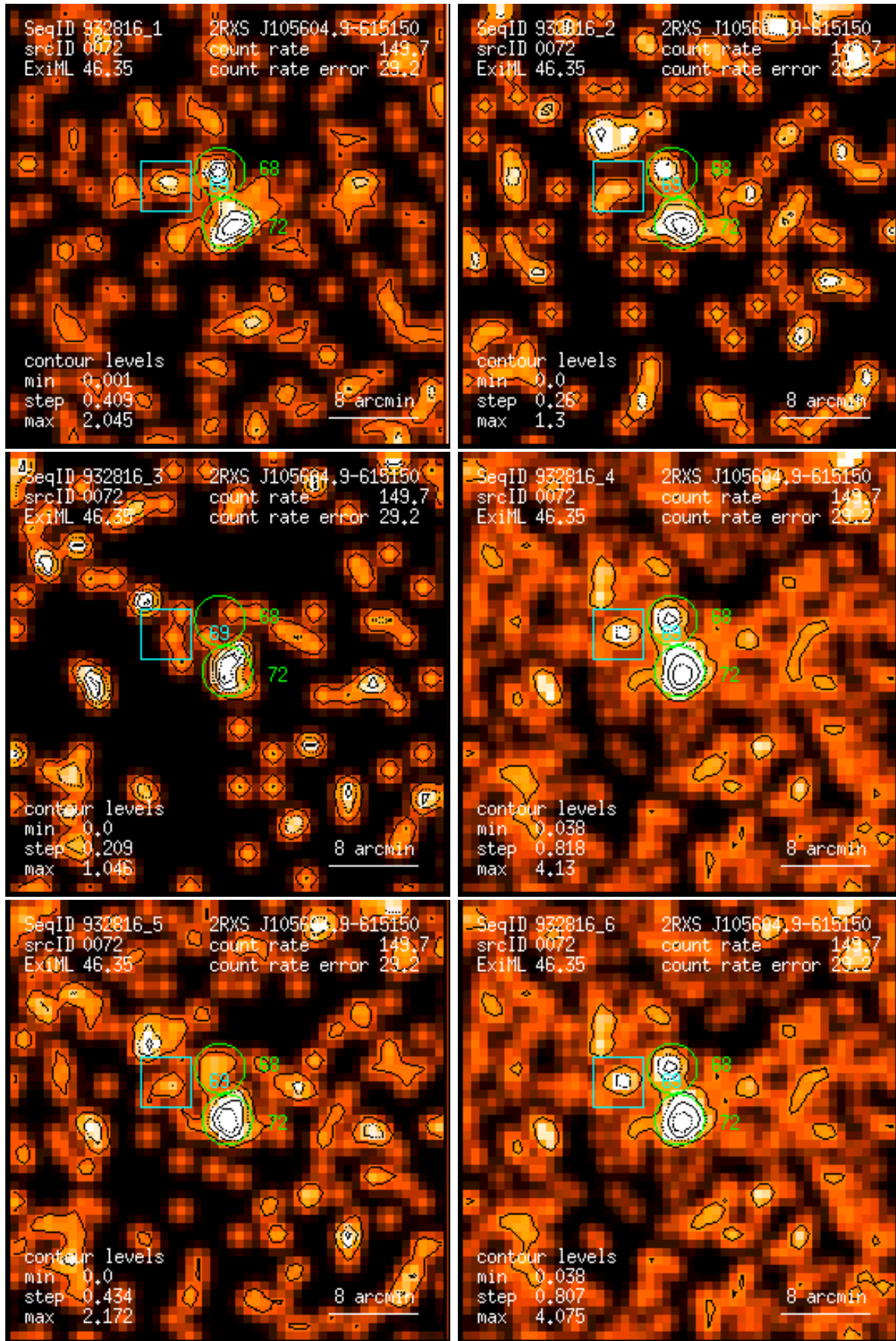
Figure 72: RASS 932816: detection 0072: band rate images, Gaussian filter: (1) PSPC channels 11 – 41, (2) 52 – 90, (3) 91 – 201, (4) 11 – 235, (5) 52 – 201, (6) 11 – 201. Broad band rates in counts/ks. Band rate contour levels in counts/ks/arcmin 2 .
