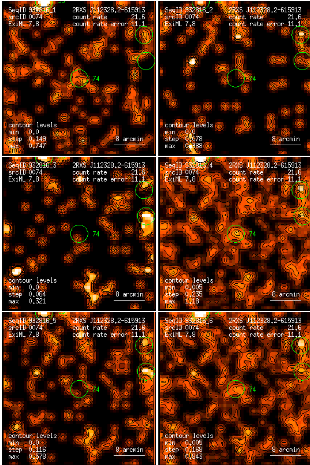
Figure 74: RASS 932816: detection 0074: band rate images, Gaussian filter: (1) PSPC channels 11 – 41, (2) 52 – 90, (3) 91 – 201, (4) 11 – 235, (5) 52 – 201, (6) 11 – 201. Broad band rates in counts/ks. Band rate contour levels in counts/ks/arcmin 2 .
