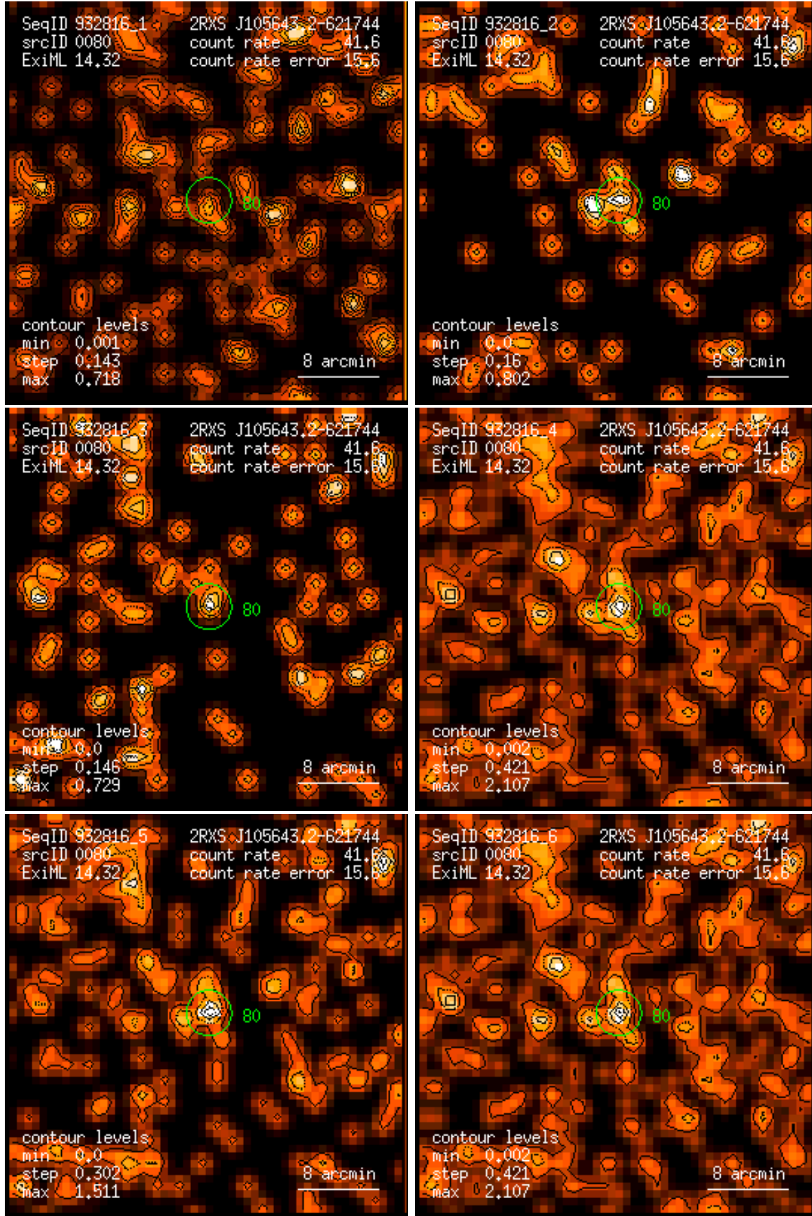
Figure 80: RASS 932816: detection 0080: band rate images, Gaussian filter: (1) PSPC channels 11 – 41, (2) 52 – 90, (3) 91 – 201, (4) 11 – 235, (5) 52 – 201, (6) 11 – 201. Broad band rates in counts/ks. Band rate contour levels in counts/ks/arcmin 2 .
