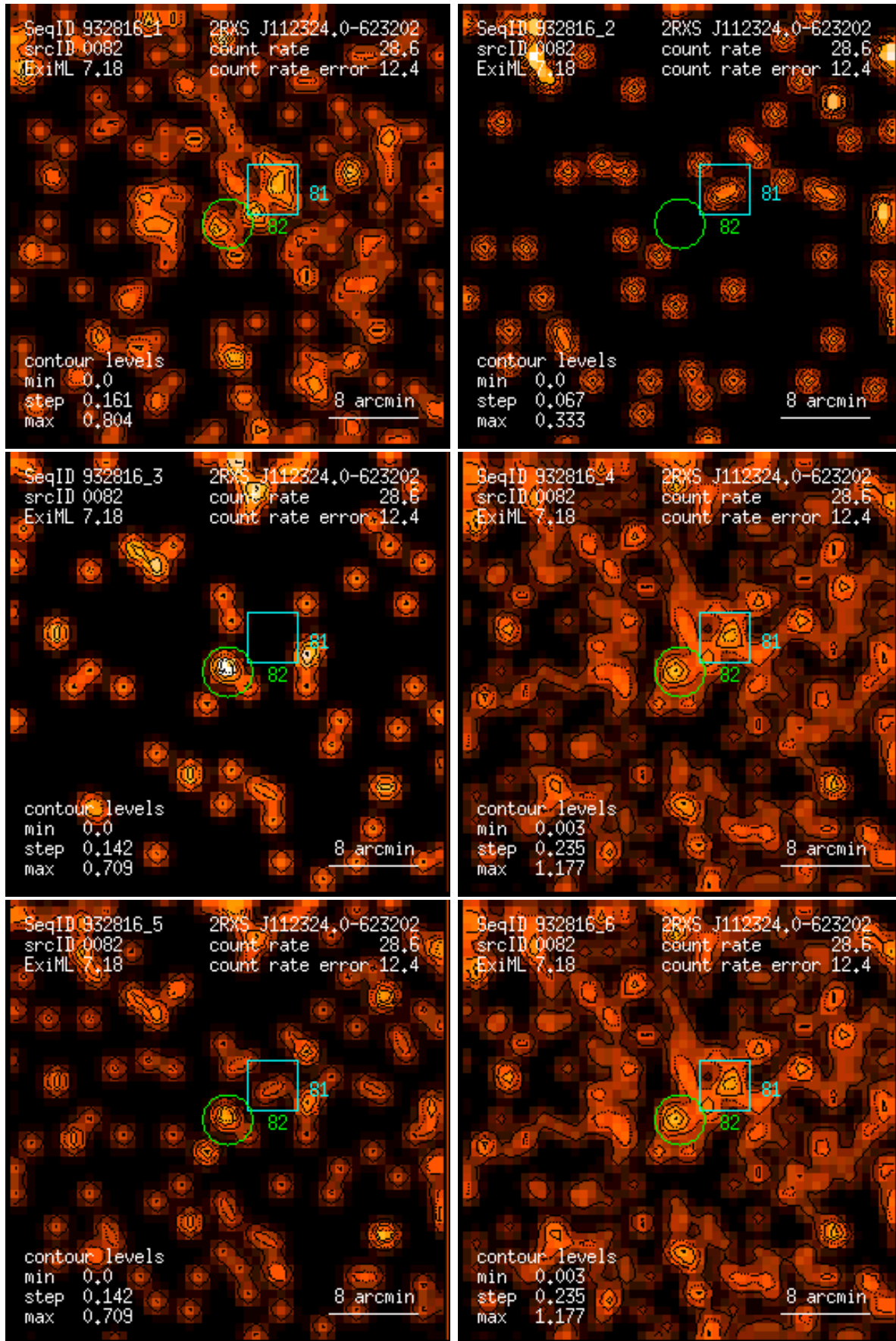
Figure 82: RASS 932816: detection 0082: band rate images, Gaussian filter: (1) PSPC channels 11 – 41, (2) 52 – 90, (3) 91 – 201, (4) 11 – 235, (5) 52 – 201, (6) 11 – 201. Broad band rates in counts/ks. Band rate contour levels in counts/ks/arcmin 2 .
