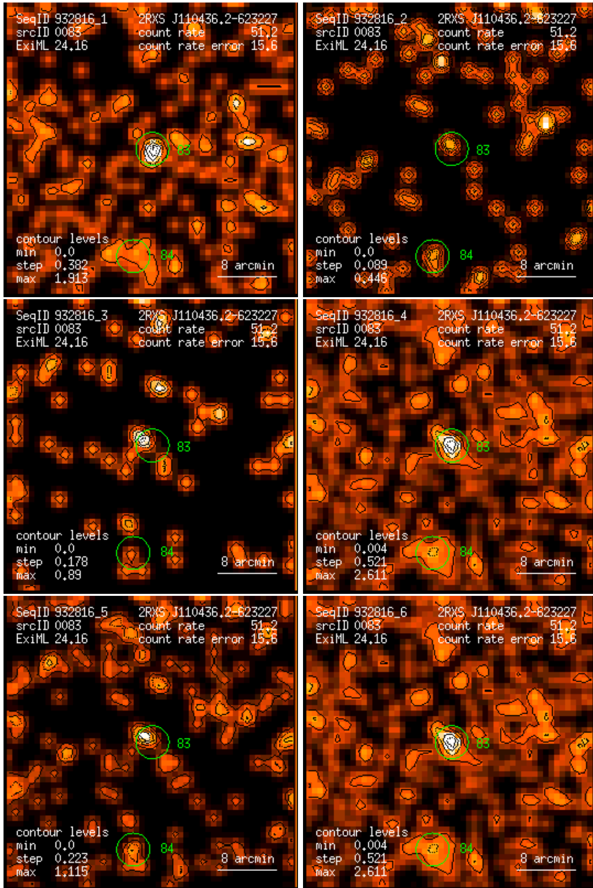
Figure 83: RASS 932816: detection 0083: band rate images, Gaussian filter: (1) PSPC channels 11 – 41, (2) 52 – 90, (3) 91 – 201, (4) 11 – 235, (5) 52 – 201, (6) 11 – 201. Broad band rates in counts/ks. Band rate contour levels in counts/ks/arcmin 2 .
