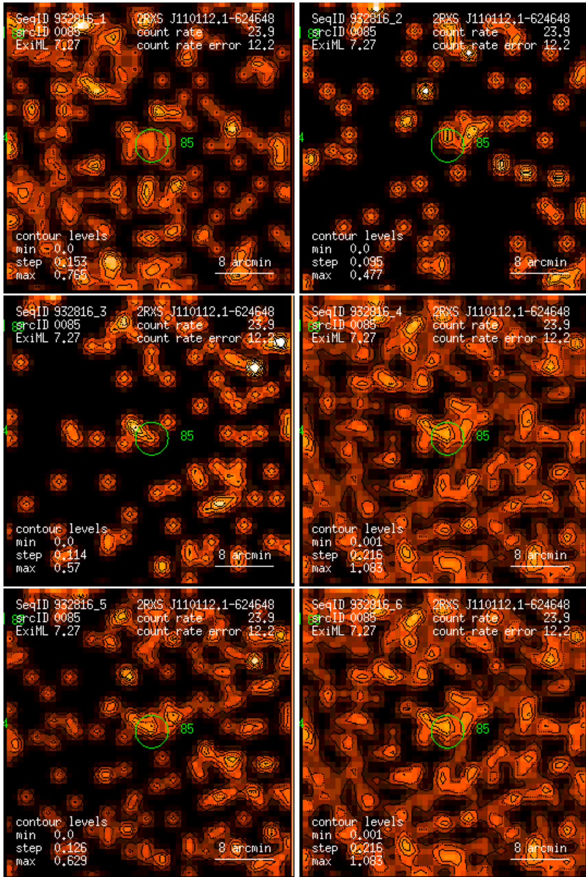
Figure 85: RASS 932816: detection 0085: band rate images, Gaussian filter: (1) PSPC channels 11 – 41, (2) 52 – 90, (3) 91 – 201, (4) 11 – 235, (5) 52 – 201, (6) 11 – 201. Broad band rates in counts/ks. Band rate contour levels in counts/ks/arcmin 2 .
