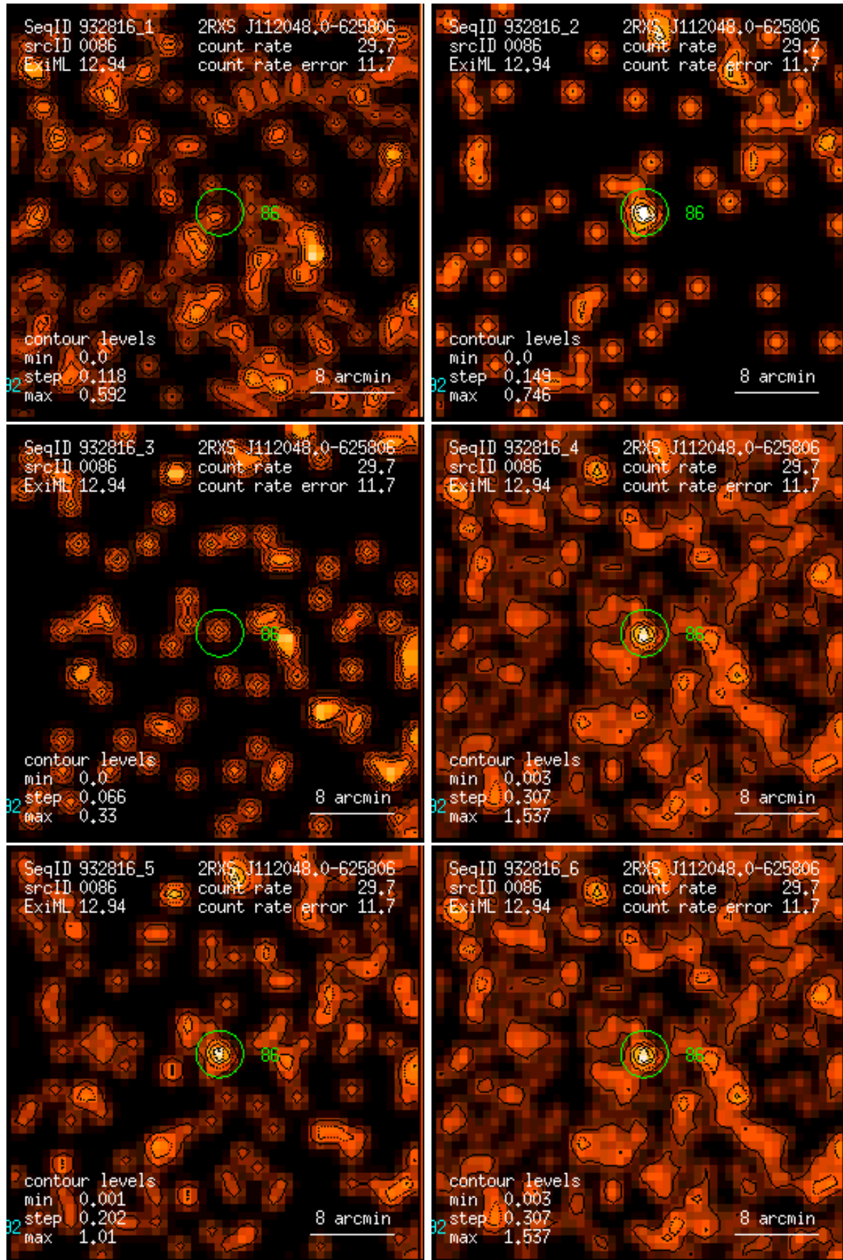
Figure 86: RASS 932816: detection 0086: band rate images, Gaussian filter: (1) PSPC channels 11 – 41, (2) 52 – 90, (3) 91 – 201, (4) 11 – 235, (5) 52 – 201, (6) 11 – 201. Broad band rates in counts/ks. Band rate contour levels in counts/ks/arcmin 2 .
