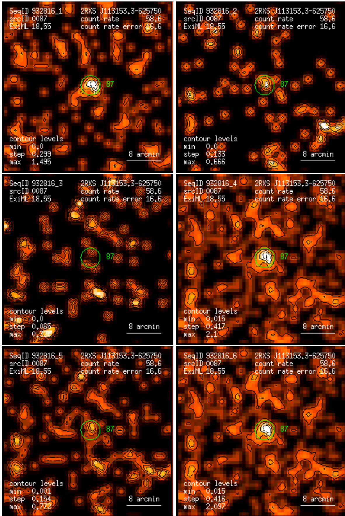
Figure 87: RASS 932816: detection 0087: band rate images, Gaussian filter: (1) PSPC channels 11 – 41, (2) 52 – 90, (3) 91 – 201, (4) 11 – 235, (5) 52 – 201, (6) 11 – 201. Broad band rates in counts/ks. Band rate contour levels in counts/ks/arcmin 2 .
