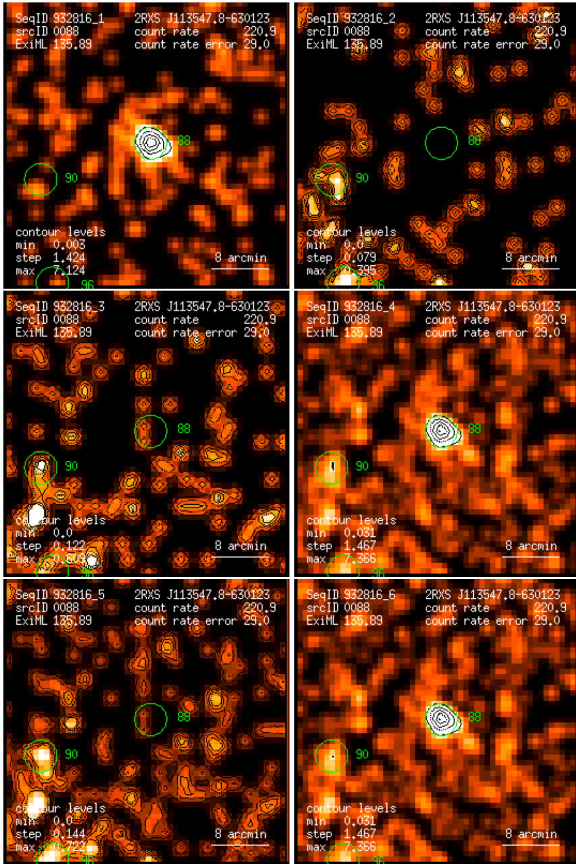
Figure 88: RASS 932816: detection 0088: band rate images, Gaussian filter: (1) PSPC channels 11 – 41, (2) 52 – 90, (3) 91 – 201, (4) 11 – 235, (5) 52 – 201, (6) 11 – 201. Broad band rates in counts/ks. Band rate contour levels in counts/ks/arcmin 2 .
