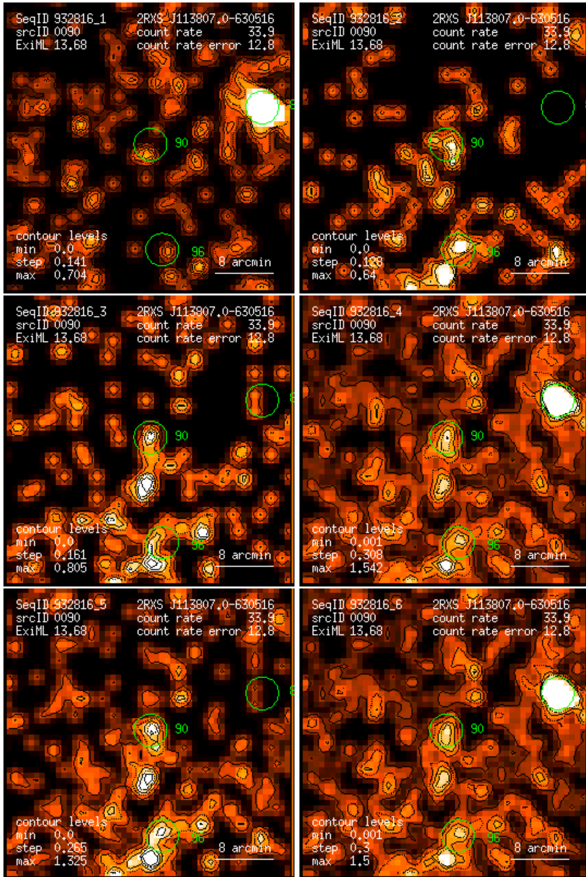
Figure 90: RASS 932816: detection 0090: band rate images, Gaussian filter: (1) PSPC channels 11 – 41, (2) 52 – 90, (3) 91 – 201, (4) 11 – 235, (5) 52 – 201, (6) 11 – 201. Broad band rates in counts/ks. Band rate contour levels in counts/ks/arcmin 2 .
