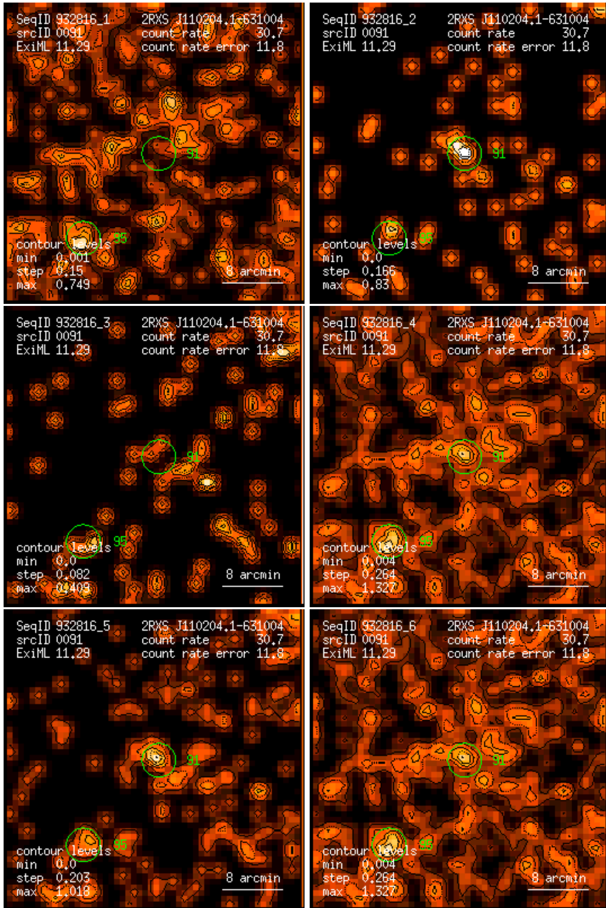
Figure 91: RASS 932816: detection 0091: band rate images, Gaussian filter: (1) PSPC channels 11 – 41, (2) 52 – 90, (3) 91 – 201, (4) 11 – 235, (5) 52 – 201, (6) 11 – 201. Broad band rates in counts/ks. Band rate contour levels in counts/ks/arcmin 2 .
