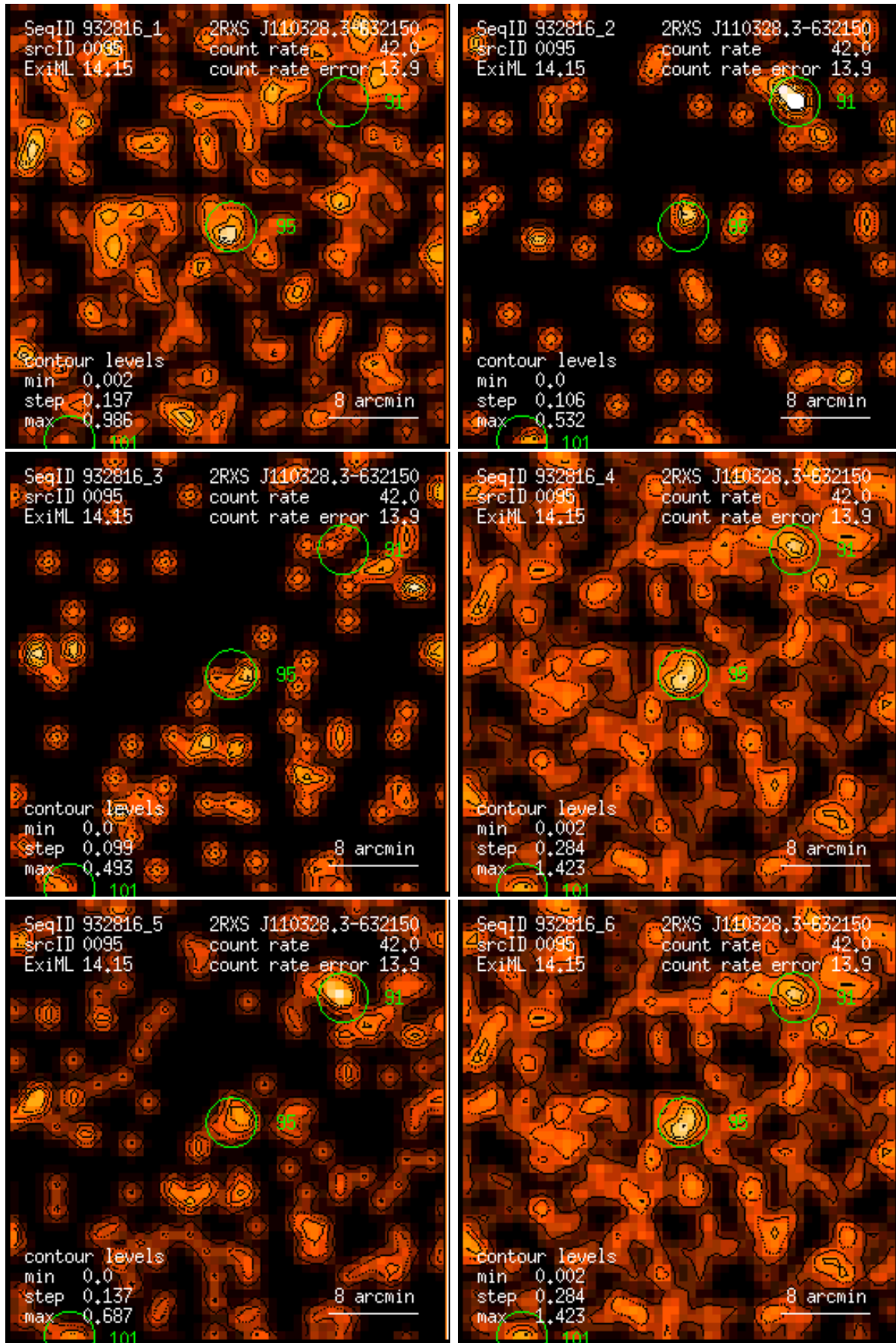
Figure 95: RASS 932816: detection 0095: band rate images, Gaussian filter: (1) PSPC channels 11 – 41, (2) 52 – 90, (3) 91 – 201, (4) 11 – 235, (5) 52 – 201, (6) 11 – 201. Broad band rates in counts/ks. Band rate contour levels in counts/ks/arcmin 2 .
