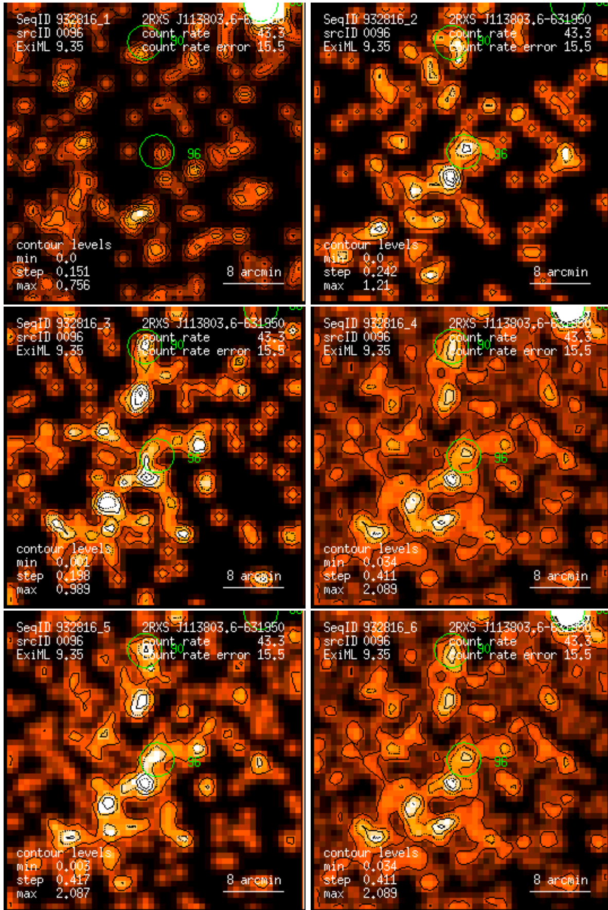
Figure 96: RASS 932816: detection 0096: band rate images, Gaussian filter: (1) PSPC channels 11 – 41, (2) 52 – 90, (3) 91 – 201, (4) 11 – 235, (5) 52 – 201, (6) 11 – 201. Broad band rates in counts/ks. Band rate contour levels in counts/ks/arcmin 2 .
