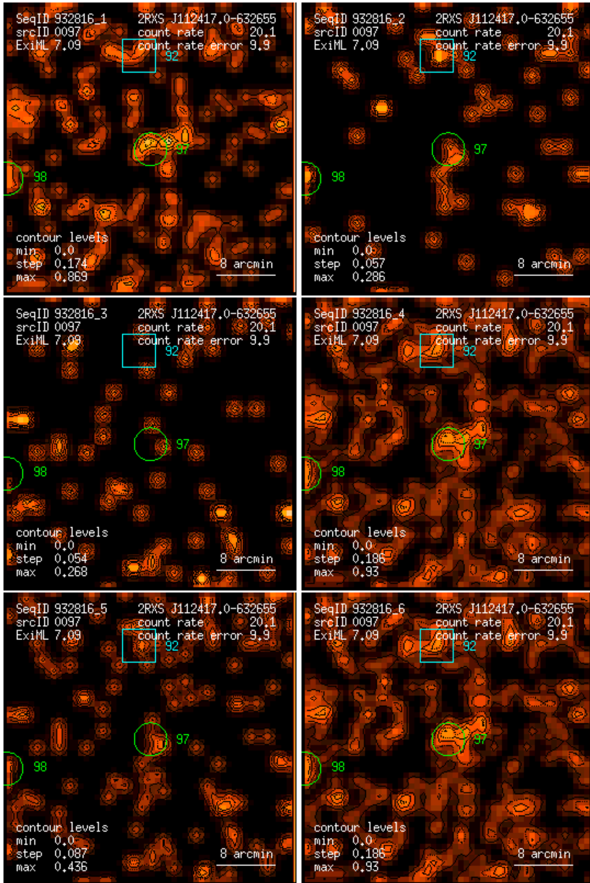
Figure 97: RASS 932816: detection 0097: band rate images, Gaussian filter: (1) PSPC channels 11 – 41, (2) 52 – 90, (3) 91 – 201, (4) 11 – 235, (5) 52 – 201, (6) 11 – 201. Broad band rates in counts/ks. Band rate contour levels in counts/ks/arcmin 2 .
