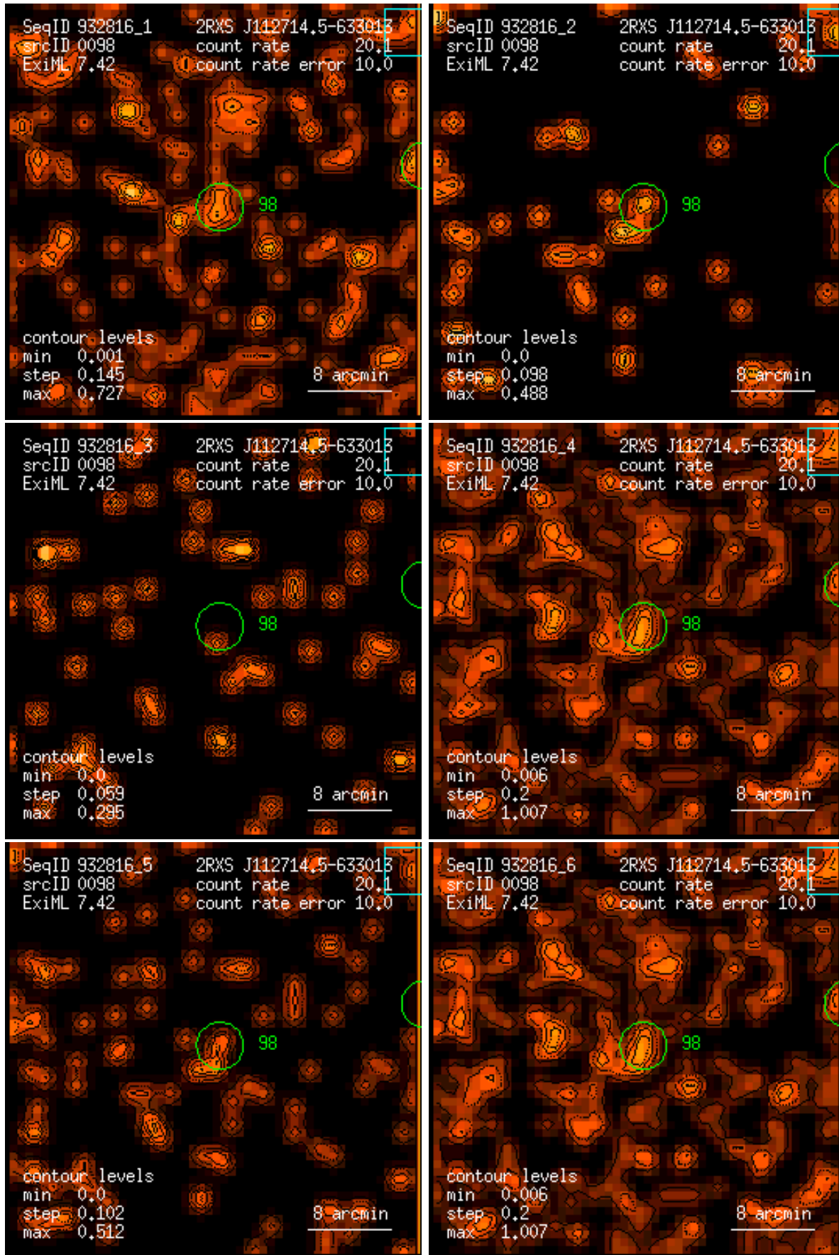
Figure 98: RASS 932816: detection 0098: band rate images, Gaussian filter: (1) PSPC channels 11 – 41, (2) 52 – 90, (3) 91 – 201, (4) 11 – 235, (5) 52 – 201, (6) 11 – 201. Broad band rates in counts/ks. Band rate contour levels in counts/ks/arcmin 2 .
