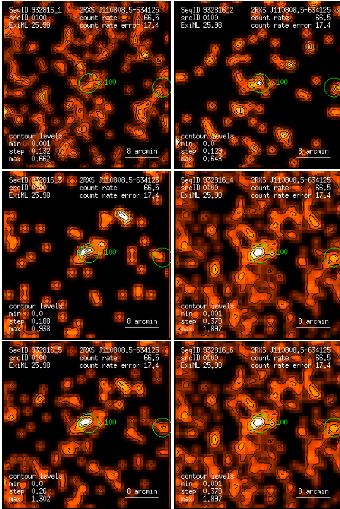
Figure 100: RASS 932816: detection 0100: band rate images, Gaussian filter: (1) PSPC channels 11 – 41, (2) 52 – 90, (3) 91 – 201, (4) 11 – 235, (5) 52 – 201, (6) 11 – 201. Broad band rates in counts/ks. Band rate contour levels in counts/ks/arcmin 2 .
