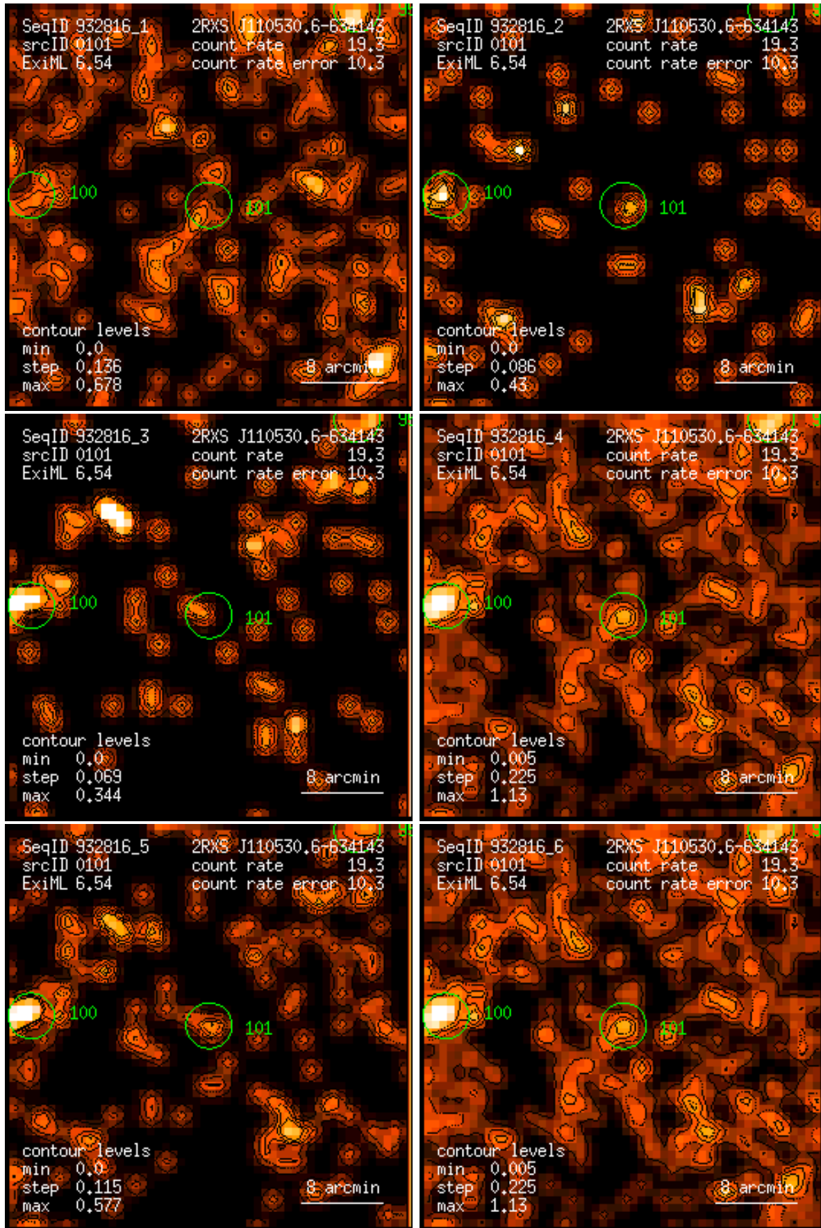
Figure 101: RASS 932816: detection 0101: band rate images, Gaussian filter: (1) PSPC channels 11 – 41, (2) 52 – 90, (3) 91 – 201, (4) 11 – 235, (5) 52 – 201, (6) 11 – 201. Broad band rates in counts/ks. Band rate contour levels in counts/ks/arcmin 2 .
