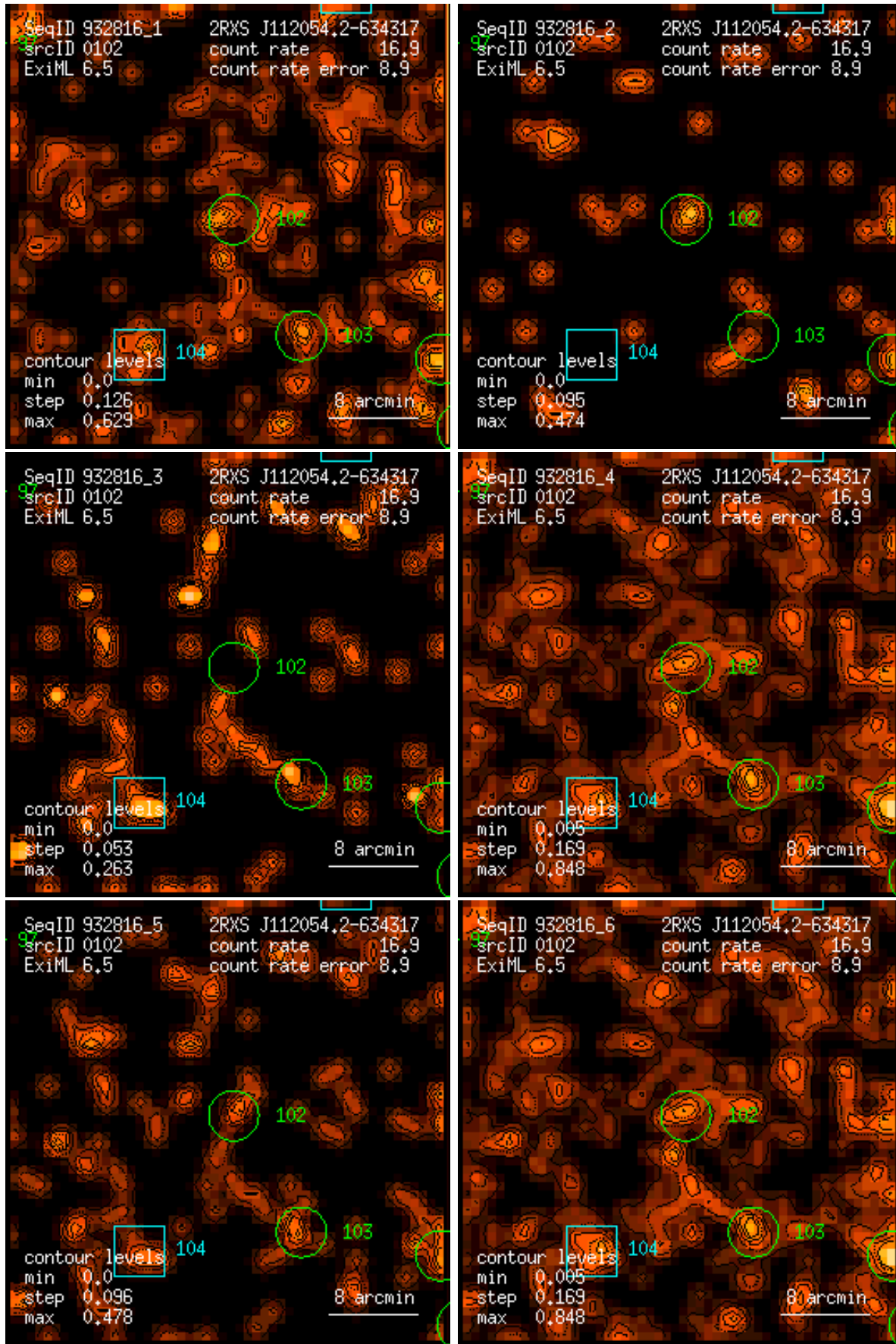
Figure 102: RASS 932816: detection 0102: band rate images, Gaussian filter: (1) PSPC channels 11 – 41, (2) 52 – 90, (3) 91 – 201, (4) 11 – 235, (5) 52 – 201, (6) 11 – 201. Broad band rates in counts/ks. Band rate contour levels in counts/ks/arcmin 2 .
