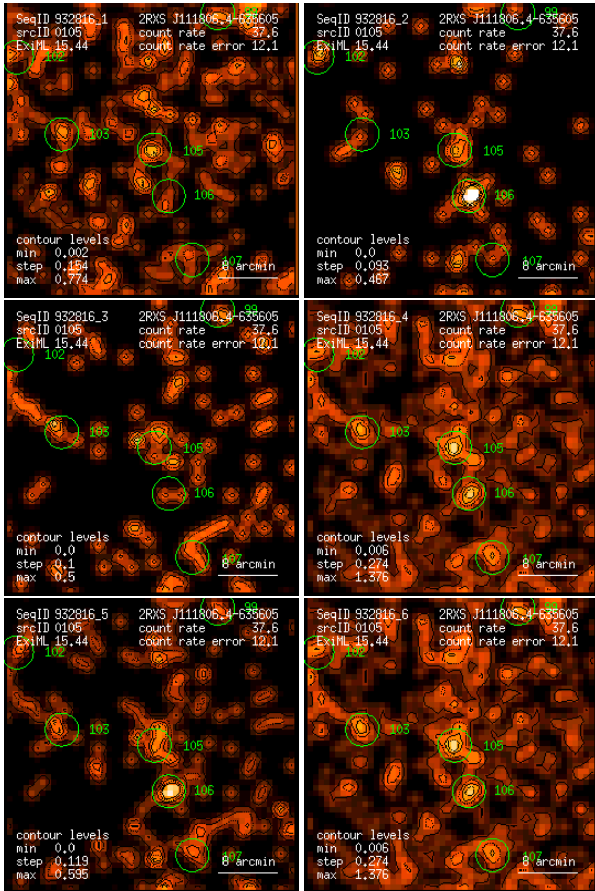
Figure 105: RASS 932816: detection 0105: band rate images, Gaussian filter: (1) PSPC channels 11 – 41, (2) 52 – 90, (3) 91 – 201, (4) 11 – 235, (5) 52 – 201, (6) 11 – 201. Broad band rates in counts/ks. Band rate contour levels in counts/ks/arcmin 2 .
