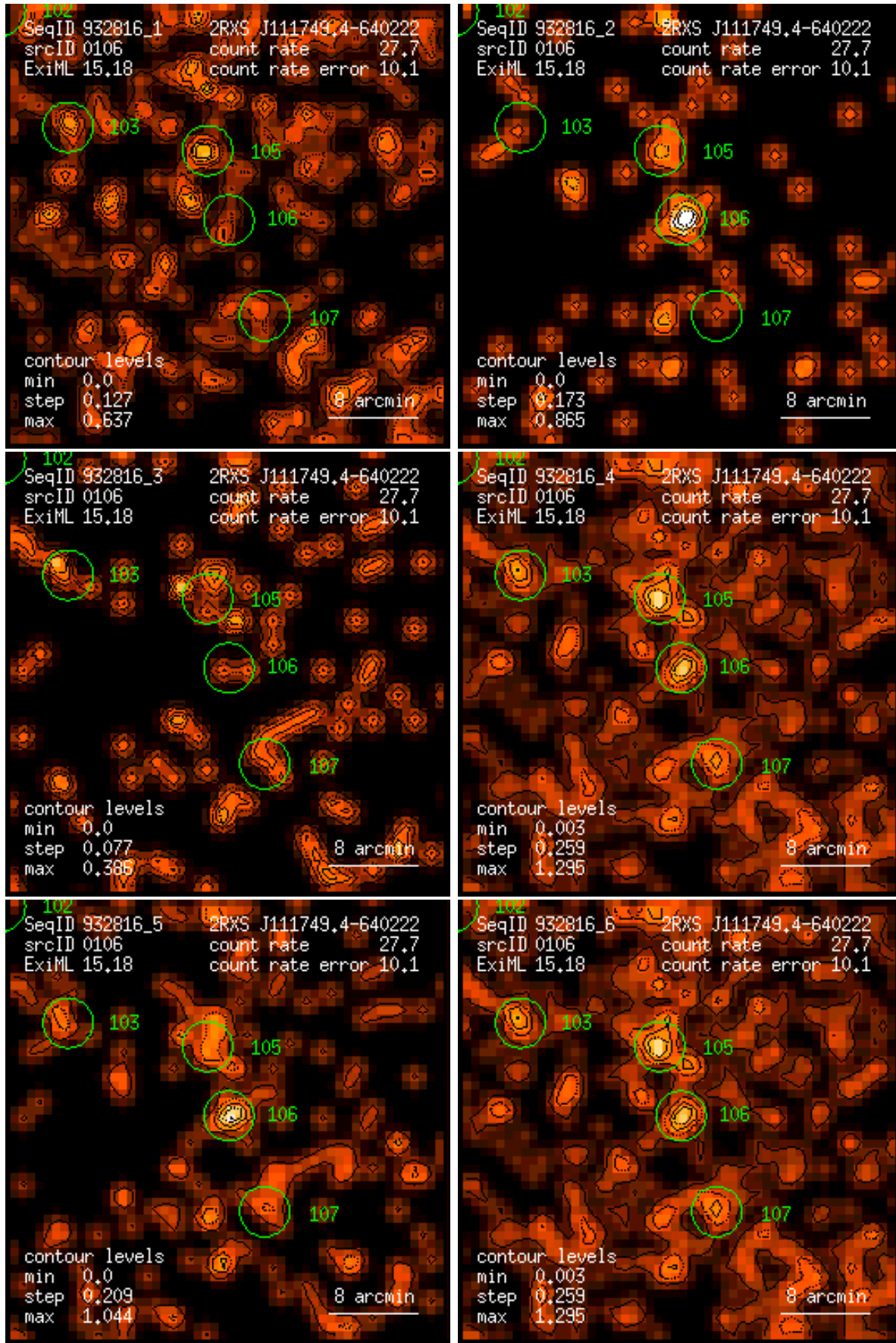
Figure 106: RASS 932816: detection 0106: band rate images, Gaussian filter: (1) PSPC channels 11 – 41, (2) 52 – 90, (3) 91 – 201, (4) 11 – 235, (5) 52 – 201, (6) 11 – 201. Broad band rates in counts/ks. Band rate contour levels in counts/ks/arcmin 2 .
