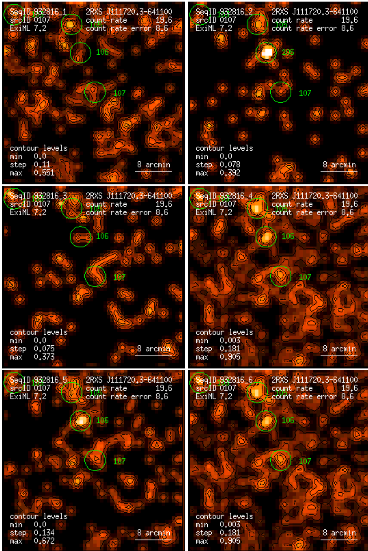
Figure 107: RASS 932816: detection 0107: band rate images, Gaussian filter: (1) PSPC channels 11 – 41, (2) 52 – 90, (3) 91 – 201, (4) 11 – 235, (5) 52 – 201, (6) 11 – 201. Broad band rates in counts/ks. Band rate contour levels in counts/ks/arcmin 2 .
