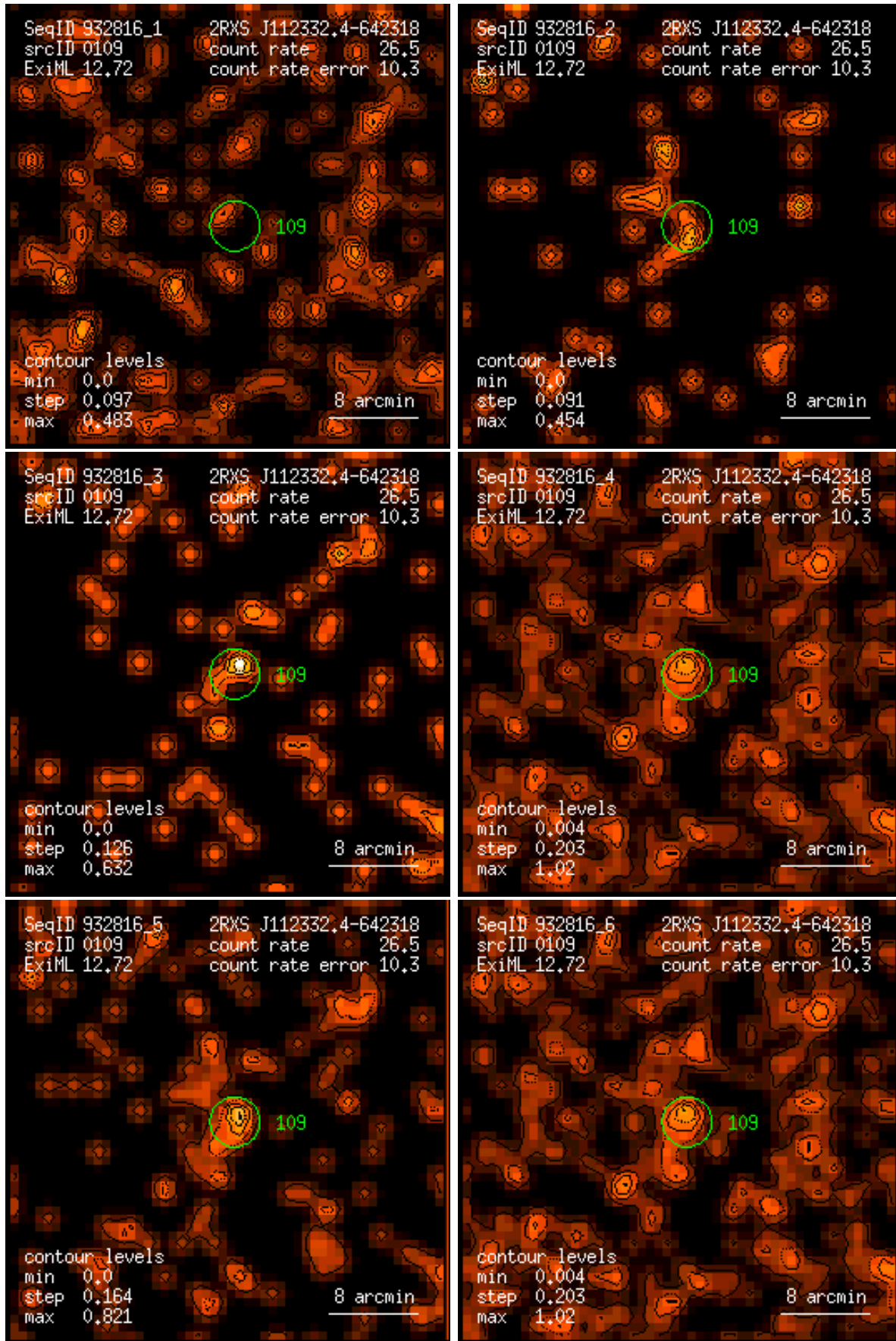
Figure 109: RASS 932816: detection 0109: band rate images, Gaussian filter: (1) PSPC channels 11 – 41, (2) 52 – 90, (3) 91 – 201, (4) 11 – 235, (5) 52 – 201, (6) 11 – 201. Broad band rates in counts/ks. Band rate contour levels in counts/ks/arcmin 2 .
