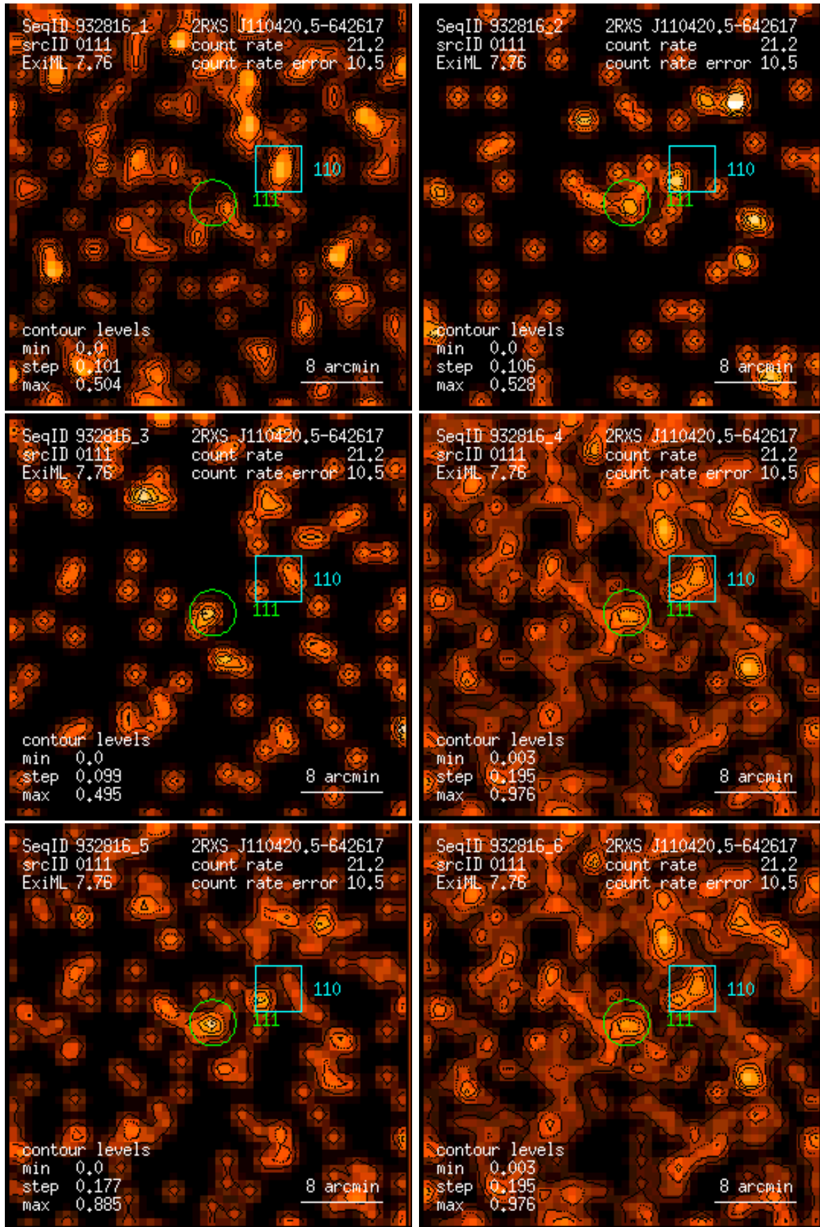
Figure 111: RASS 932816: detection 0111: band rate images, Gaussian filter: (1) PSPC channels 11 – 41, (2) 52 – 90, (3) 91 – 201, (4) 11 – 235, (5) 52 – 201, (6) 11 – 201. Broad band rates in counts/ks. Band rate contour levels in counts/ks/arcmin 2 .
