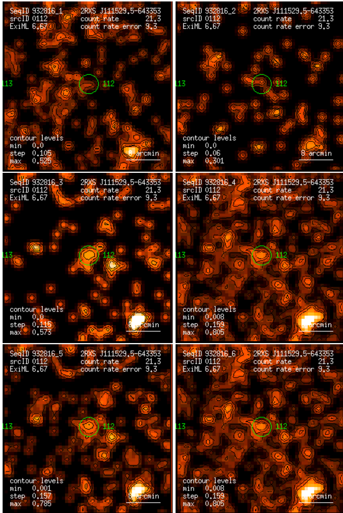
Figure 112: RASS 932816: detection 0112: band rate images, Gaussian filter: (1) PSPC channels 11 – 41, (2) 52 – 90, (3) 91 – 201, (4) 11 – 235, (5) 52 – 201, (6) 11 – 201. Broad band rates in counts/ks. Band rate contour levels in counts/ks/arcmin 2 .
