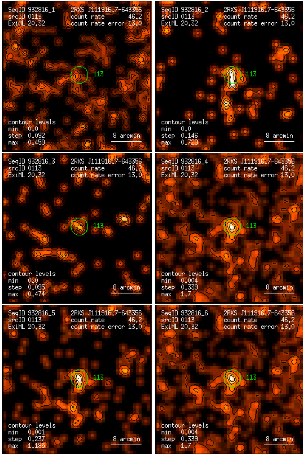
Figure 113: RASS 932816: detection 0113: band rate images, Gaussian filter: (1) PSPC channels 11 – 41, (2) 52 – 90, (3) 91 – 201, (4) 11 – 235, (5) 52 – 201, (6) 11 – 201. Broad band rates in counts/ks. Band rate contour levels in counts/ks/arcmin 2 .
