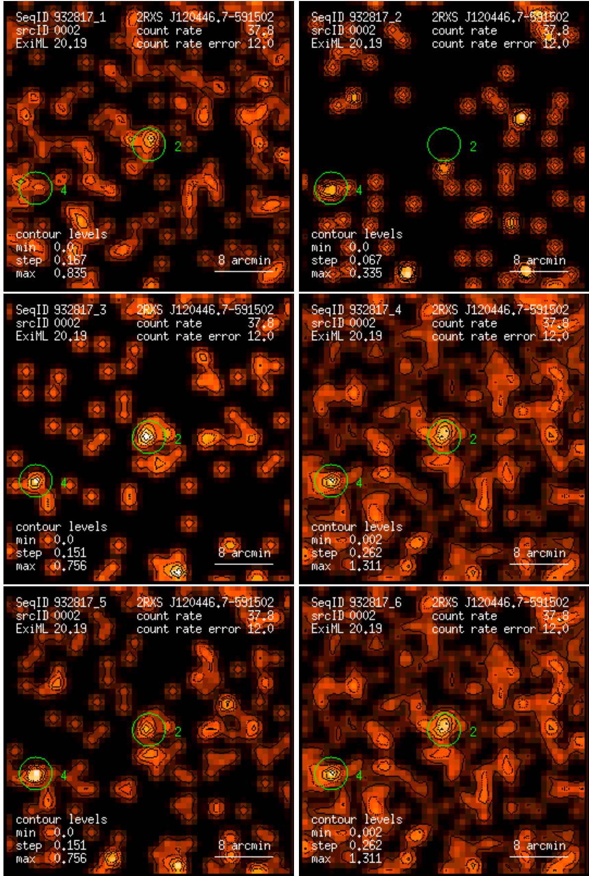
Figure 2: RASS 932817: detection 0002: band rate images, Gaussian filter: (1) PSPC channels 11 – 41, (2) 52 – 90, (3) 91 – 201, (4) 11 – 235, (5) 52 – 201, (6) 11 – 201. Broad band rates in counts/ks. Band rate contour levels in counts/ks/arcmin 2 .
