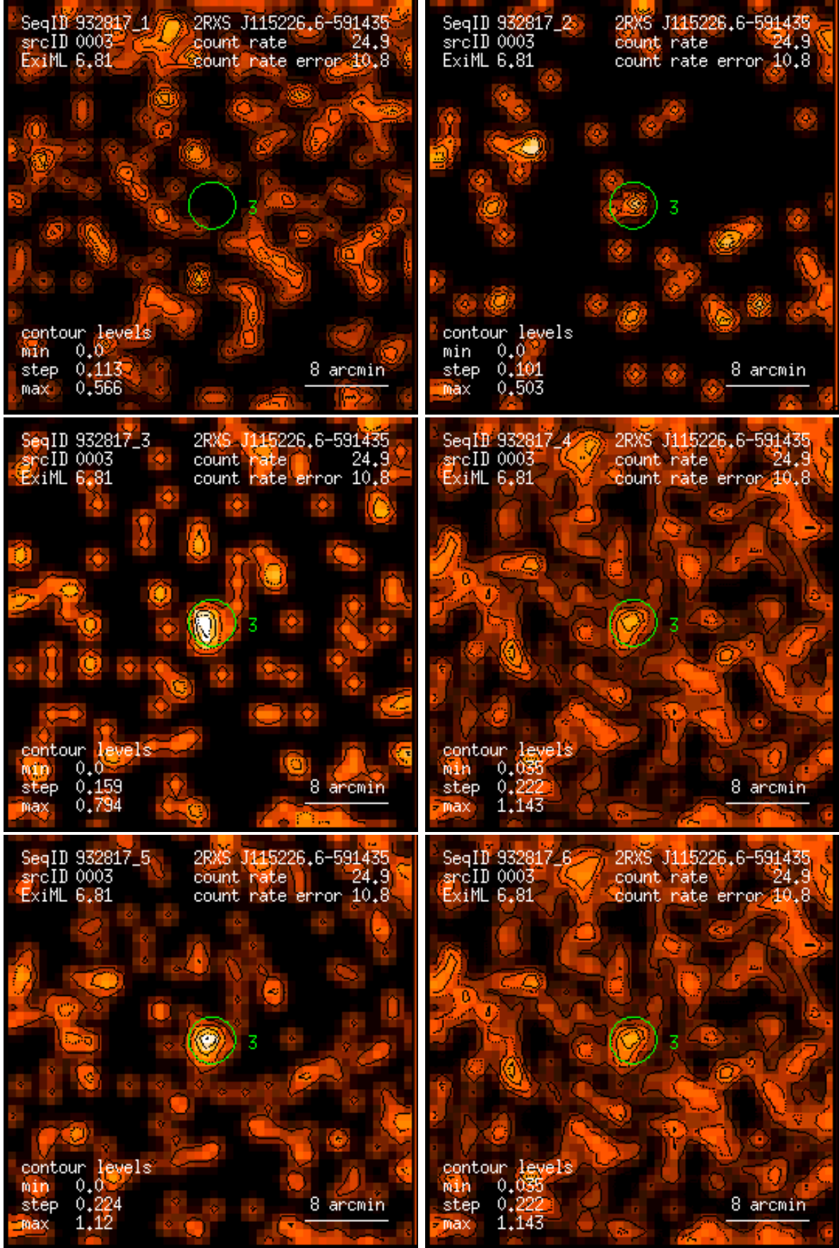
Figure 3: RASS 932817: detection 0003: band rate images, Gaussian filter: (1) PSPC channels 11 – 41, (2) 52 – 90, (3) 91 – 201, (4) 11 – 235, (5) 52 – 201, (6) 11 – 201. Broad band rates in counts/ks. Band rate contour levels in counts/ks/arcmin 2 .
