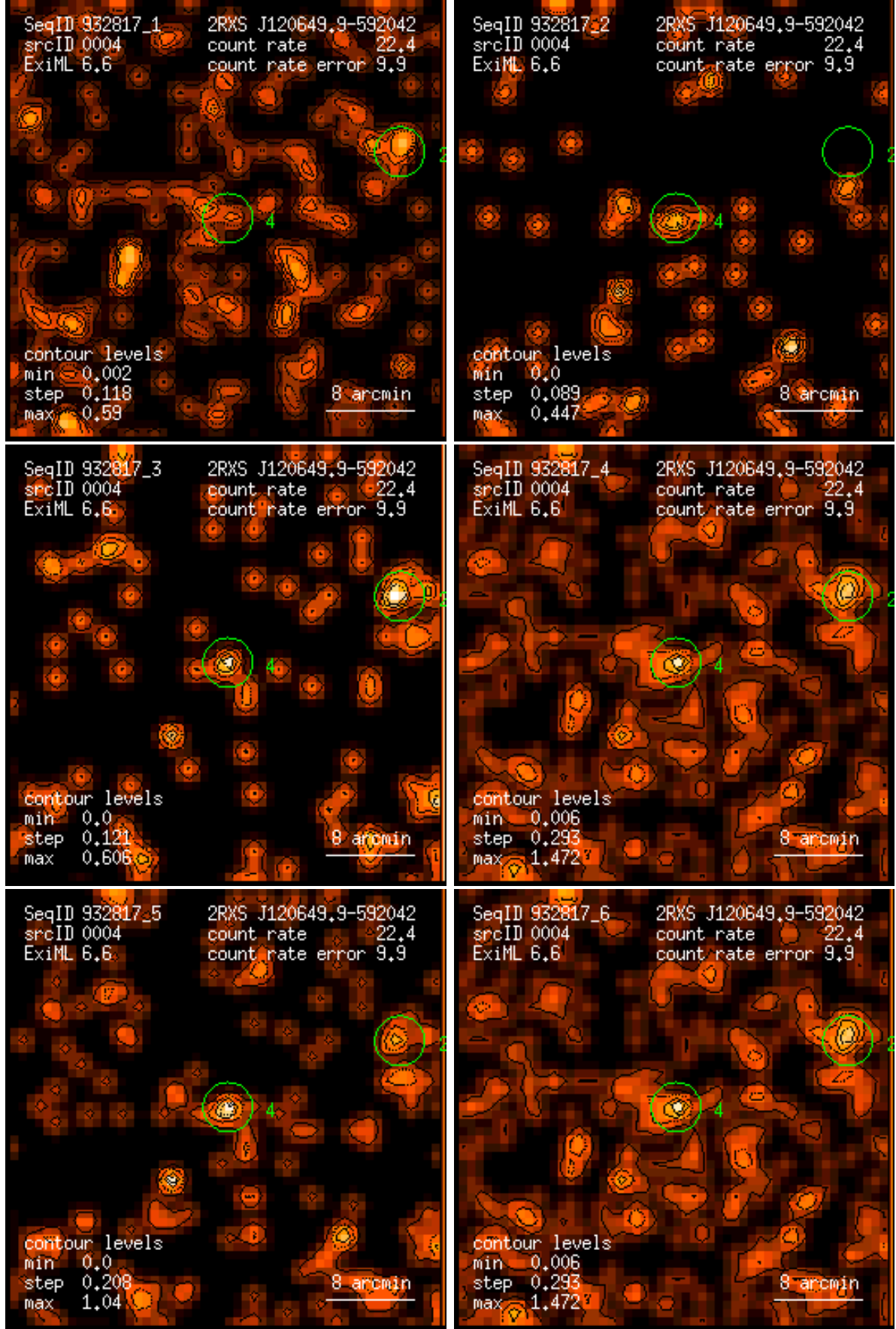
Figure 4: RASS 932817: detection 0004: band rate images, Gaussian filter: (1) PSPC channels 11 – 41, (2) 52 – 90, (3) 91 – 201, (4) 11 – 235, (5) 52 – 201, (6) 11 – 201. Broad band rates in counts/ks. Band rate contour levels in counts/ks/arcmin 2 .
