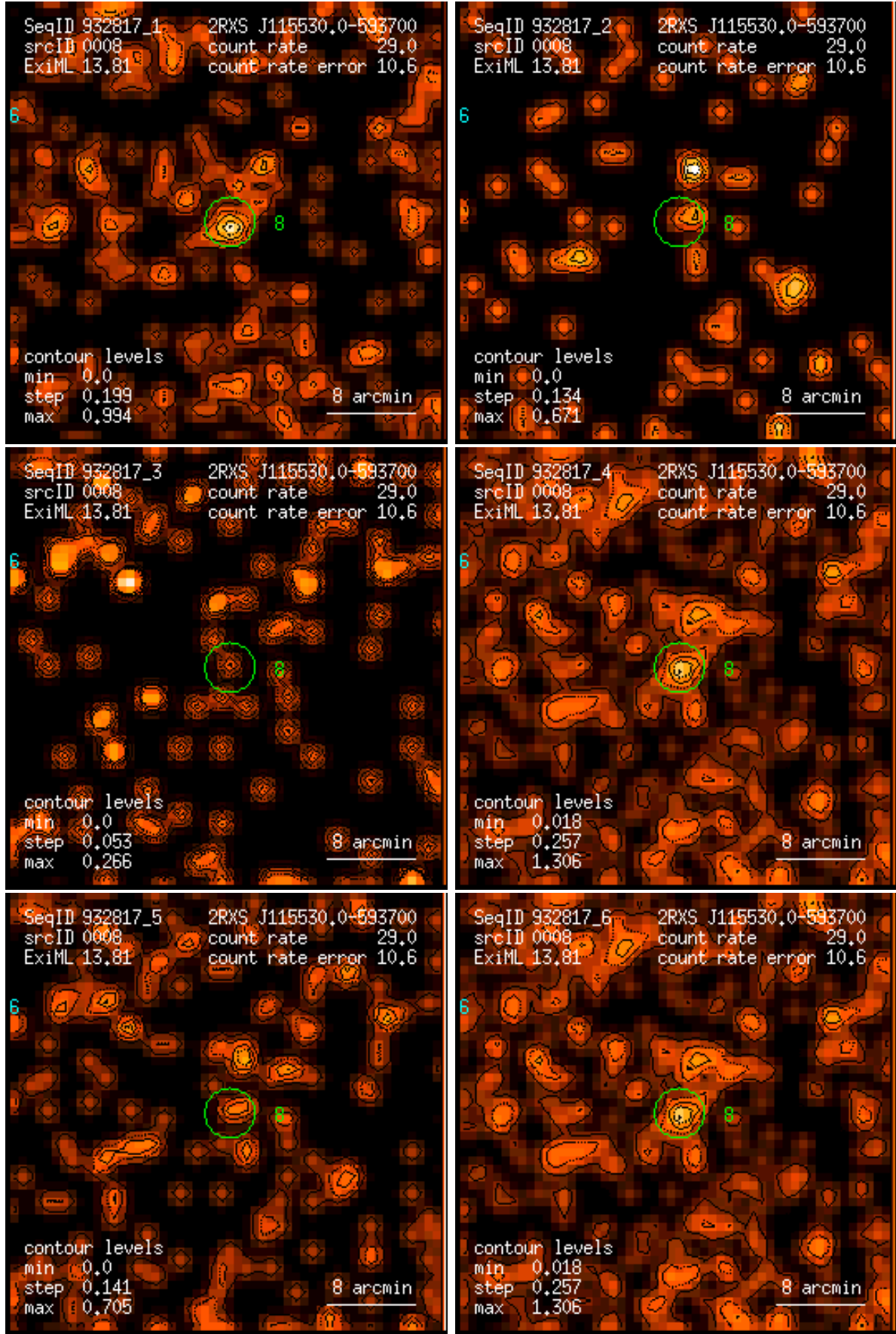
Figure 8: RASS 932817: detection 0008: band rate images, Gaussian filter: (1) PSPC channels 11 – 41, (2) 52 – 90, (3) 91 – 201, (4) 11 – 235, (5) 52 – 201, (6) 11 – 201. Broad band rates in counts/ks. Band rate contour levels in counts/ks/arcmin 2 .
